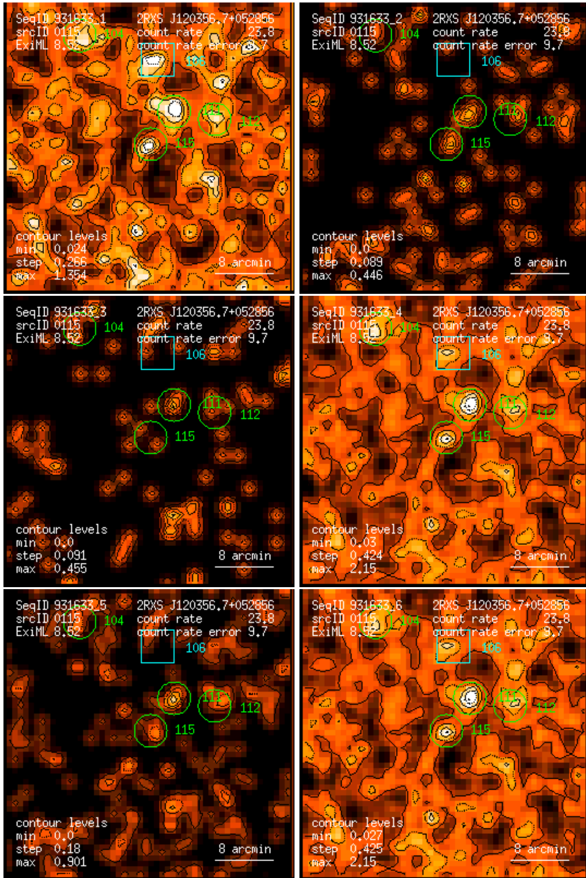
Figure 115: RASS 931633: detection 0115: band rate images, Gaussian filter: (1) PSPC channels 11 – 41, (2) 52 – 90, (3) 91 – 201, (4) 11 – 235, (5) 52 – 201, (6) 11 – 201. Broad band rates in counts/ks. Band rate contour levels in counts/ks/arcmin 2 .
