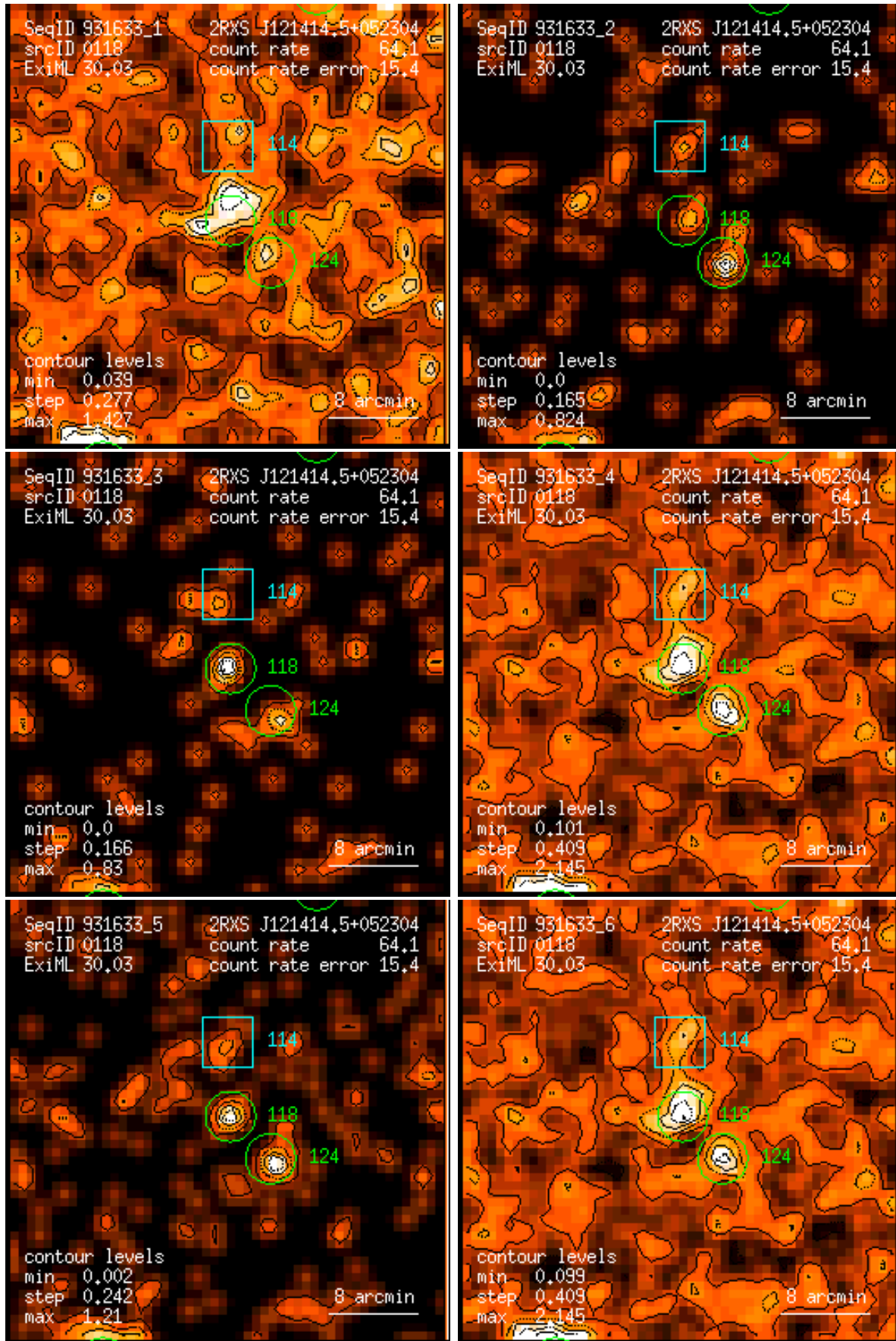
Figure 118: RASS 931633: detection 0118: band rate images, Gaussian filter: (1) PSPC channels 11 – 41, (2) 52 – 90, (3) 91 – 201, (4) 11 – 235, (5) 52 – 201, (6) 11 – 201. Broad band rates in counts/ks. Band rate contour levels in counts/ks/arcmin 2 .
