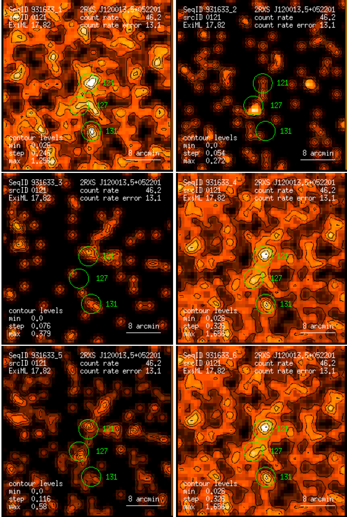
Figure 121: RASS 931633: detection 0121: band rate images, Gaussian filter: (1) PSPC channels 11 – 41, (2) 52 – 90, (3) 91 – 201, (4) 11 – 235, (5) 52 – 201, (6) 11 – 201. Broad band rates in counts/ks. Band rate contour levels in counts/ks/arcmin 2 .
