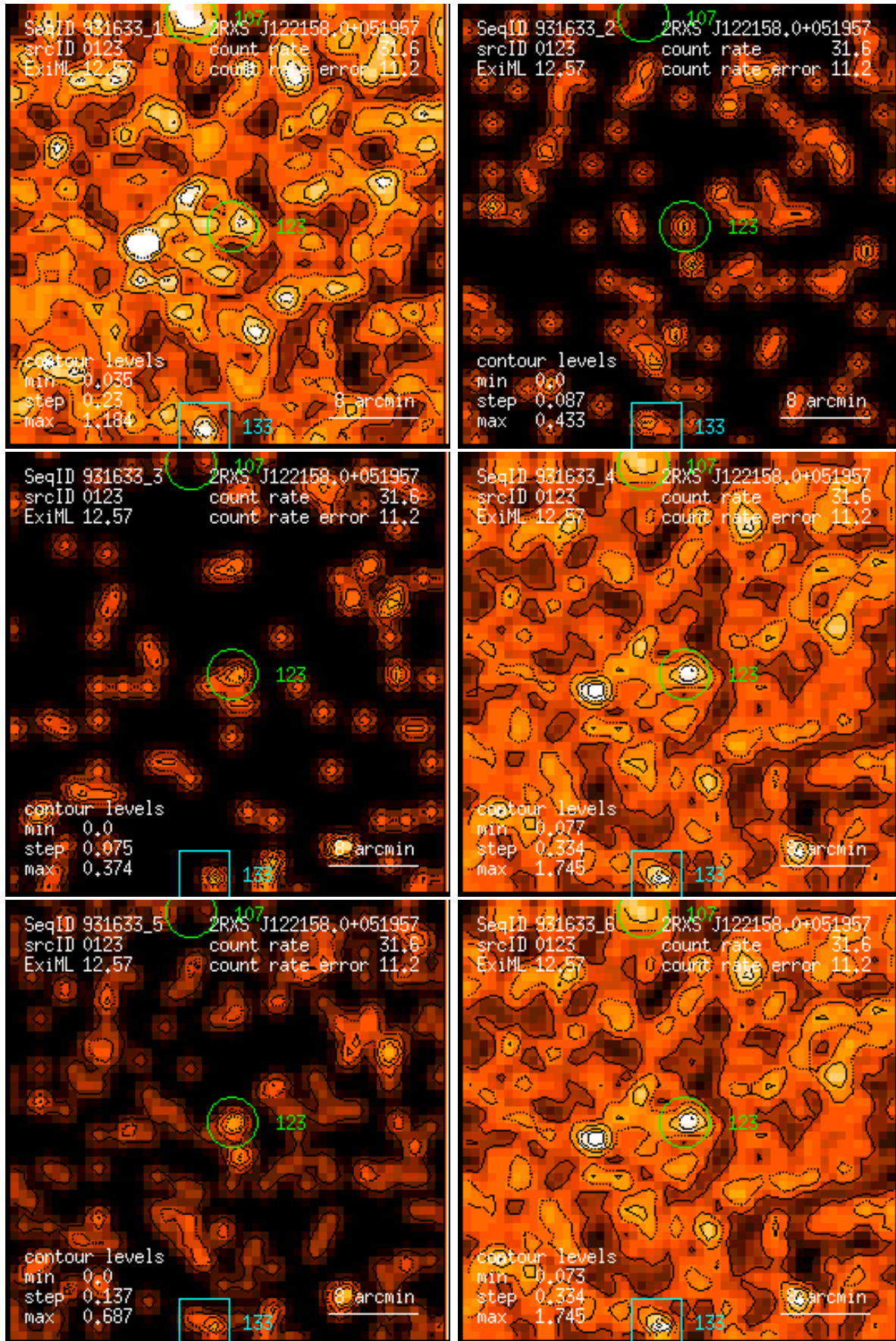
Figure 123: RASS 931633: detection 0123: band rate images, Gaussian filter: (1) PSPC channels 11 – 41, (2) 52 – 90, (3) 91 – 201, (4) 11 – 235, (5) 52 – 201, (6) 11 – 201. Broad band rates in counts/ks. Band rate contour levels in counts/ks/arcmin 2 .
