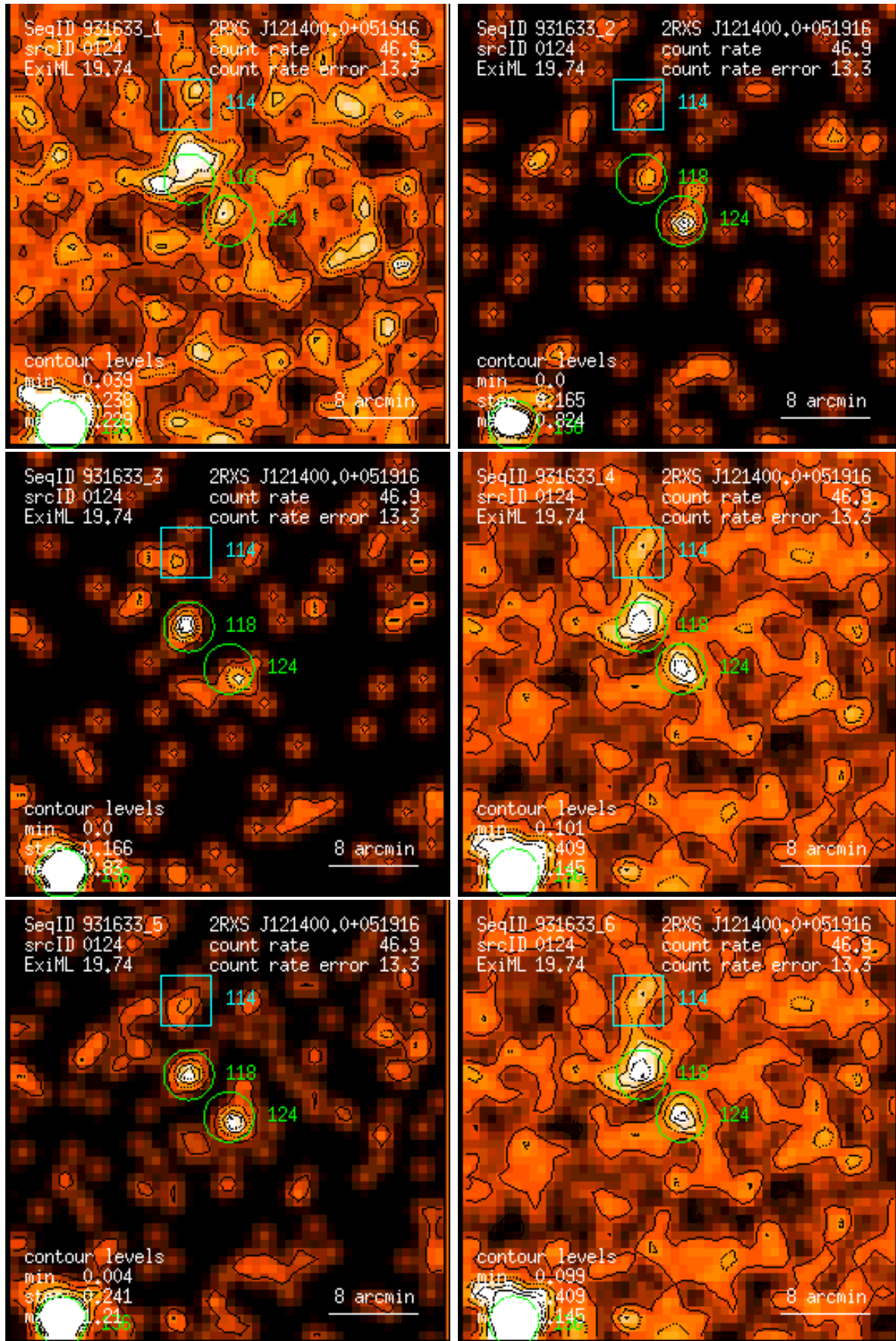
Figure 124: RASS 931633: detection 0124: band rate images, Gaussian filter: (1) PSPC channels 11 – 41, (2) 52 – 90, (3) 91 – 201, (4) 11 – 235, (5) 52 – 201, (6) 11 – 201. Broad band rates in counts/ks. Band rate contour levels in counts/ks/arcmin 2 .
