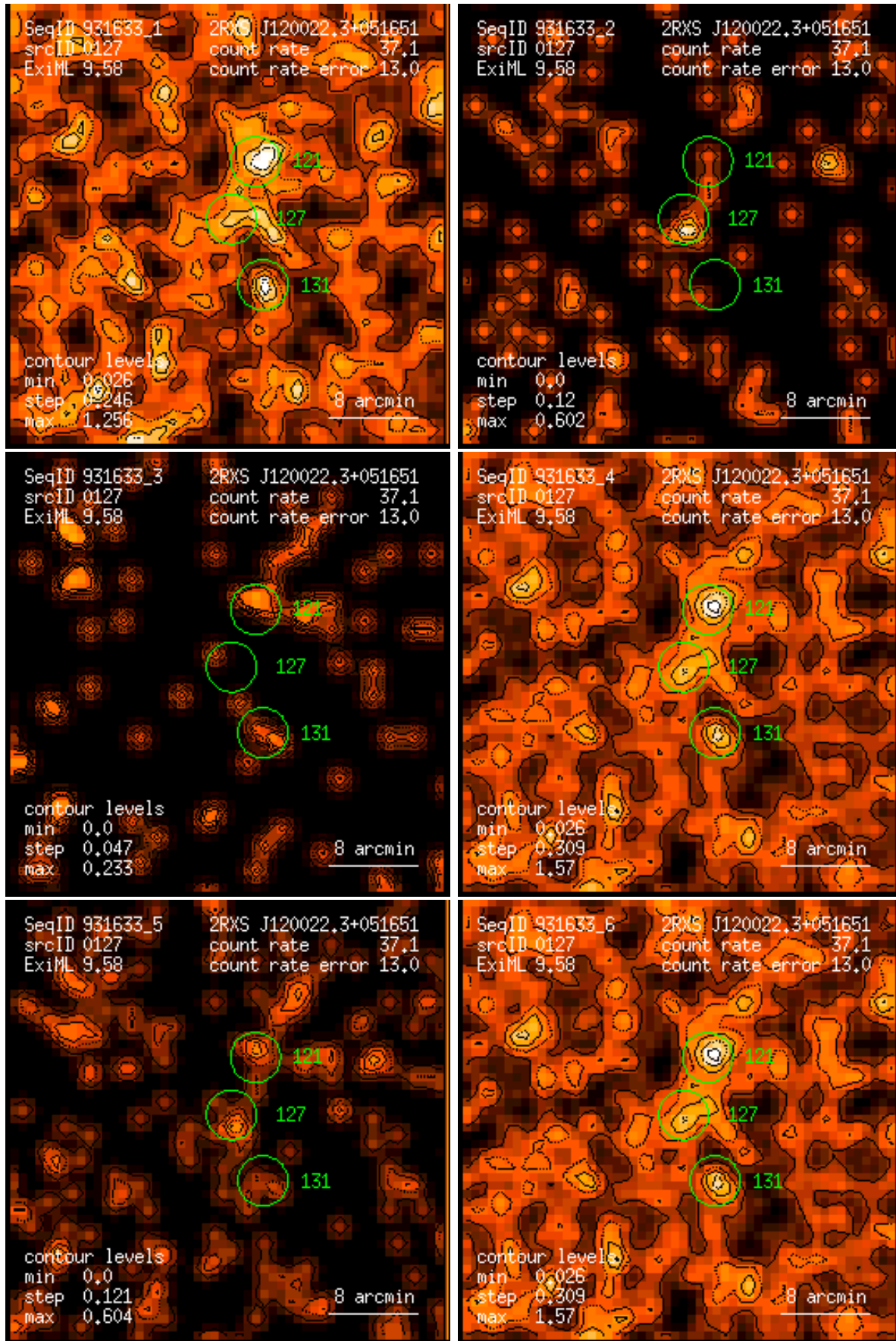
Figure 127: RASS 931633: detection 0127: band rate images, Gaussian filter: (1) PSPC channels 11 – 41, (2) 52 – 90, (3) 91 – 201, (4) 11 – 235, (5) 52 – 201, (6) 11 – 201. Broad band rates in counts/ks. Band rate contour levels in counts/ks/arcmin 2 .
