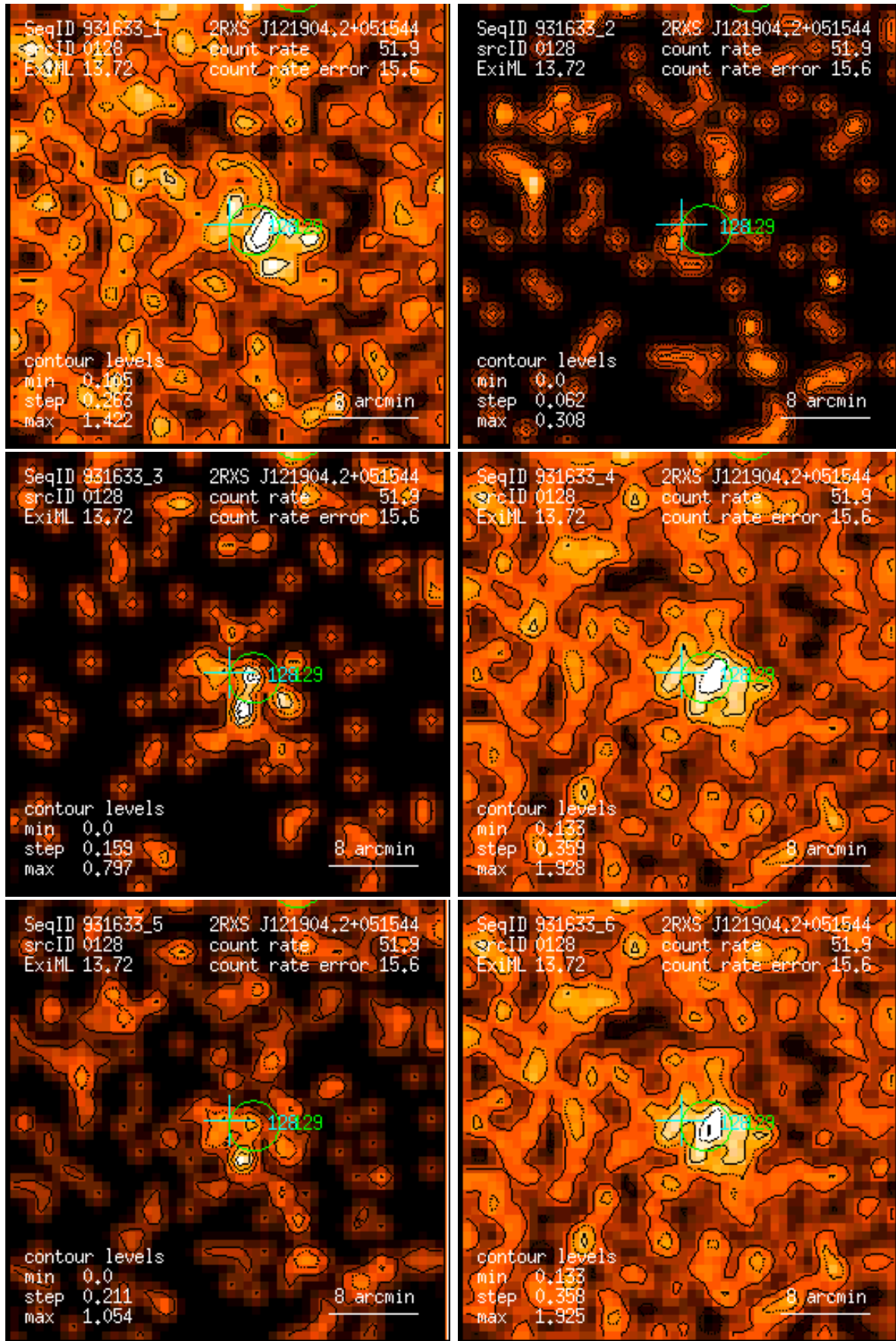
Figure 128: RASS 931633: detection 0128: band rate images, Gaussian filter: (1) PSPC channels 11 – 41, (2) 52 – 90, (3) 91 – 201, (4) 11 – 235, (5) 52 – 201, (6) 11 – 201. Broad band rates in counts/ks. Band rate contour levels in counts/ks/arcmin 2 .
