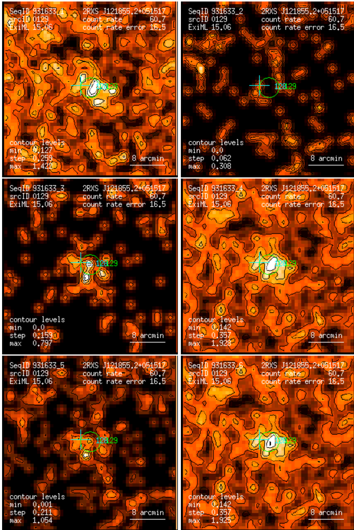
Figure 129: RASS 931633: detection 0129: band rate images, Gaussian filter: (1) PSPC channels 11 – 41, (2) 52 – 90, (3) 91 – 201, (4) 11 – 235, (5) 52 – 201, (6) 11 – 201. Broad band rates in counts/ks. Band rate contour levels in counts/ks/arcmin 2 .
