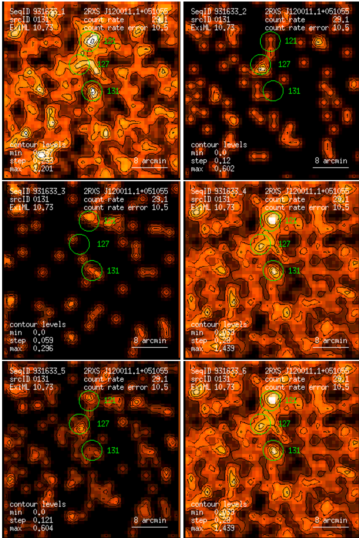
Figure 131: RASS 931633: detection 0131: band rate images, Gaussian filter: (1) PSPC channels 11 – 41, (2) 52 – 90, (3) 91 – 201, (4) 11 – 235, (5) 52 – 201, (6) 11 – 201. Broad band rates in counts/ks. Band rate contour levels in counts/ks/arcmin 2 .
