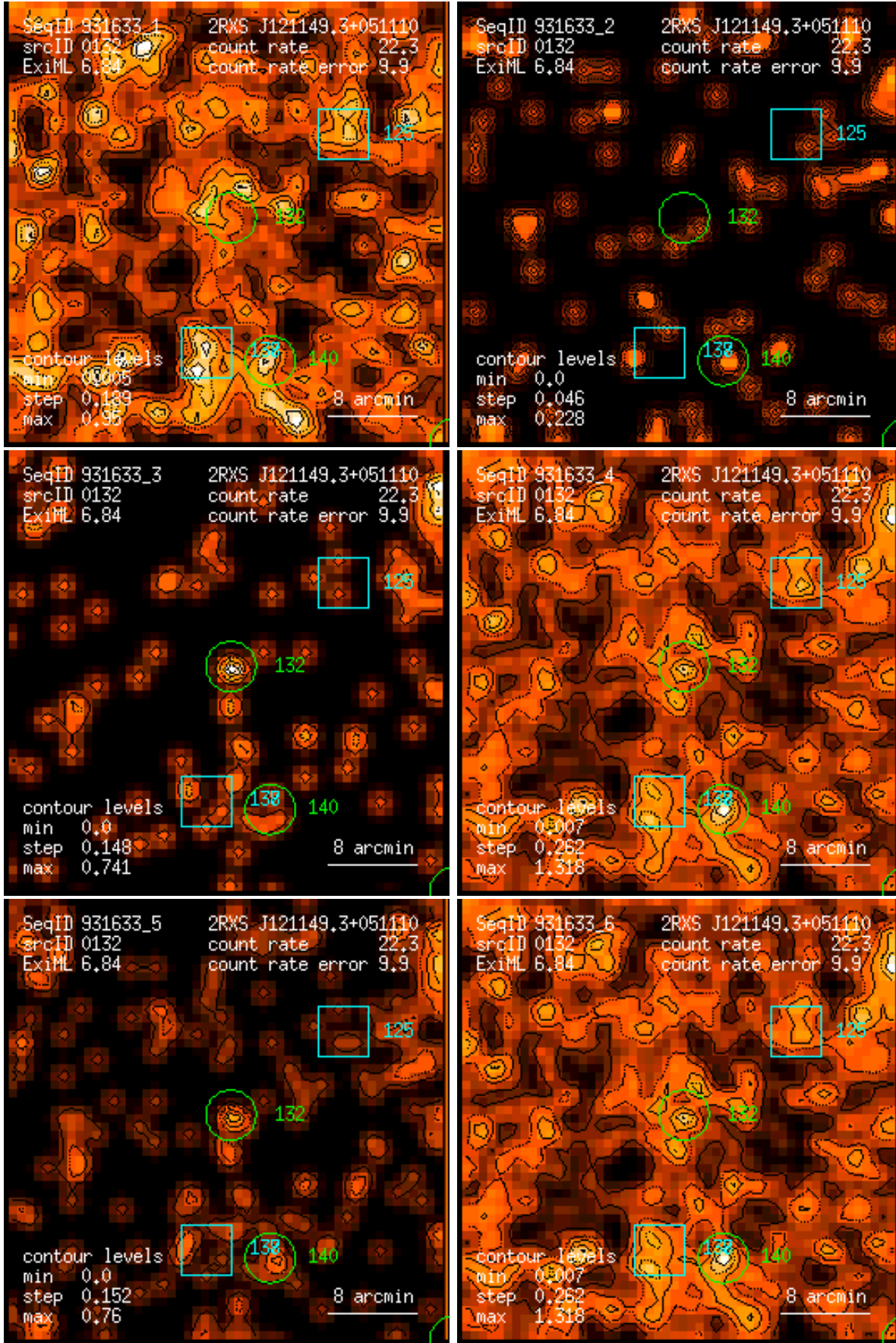
Figure 132: RASS 931633: detection 0132: band rate images, Gaussian filter: (1) PSPC channels 11 – 41, (2) 52 – 90, (3) 91 – 201, (4) 11 – 235, (5) 52 – 201, (6) 11 – 201. Broad band rates in counts/ks. Band rate contour levels in counts/ks/arcmin 2 .
