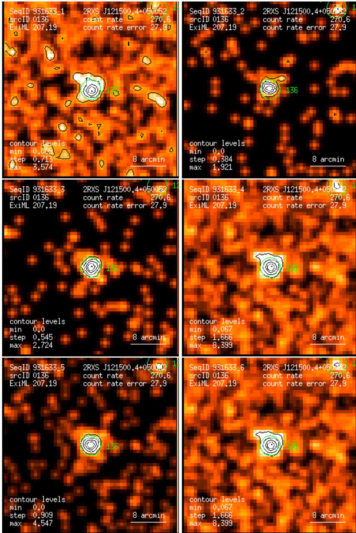
Figure 136: RASS 931633: detection 0136: band rate images, Gaussian filter: (1) PSPC channels 11 – 41, (2) 52 – 90, (3) 91 – 201, (4) 11 – 235, (5) 52 – 201, (6) 11 – 201. Broad band rates in counts/ks. Band rate contour levels in counts/ks/arcmin 2 .
