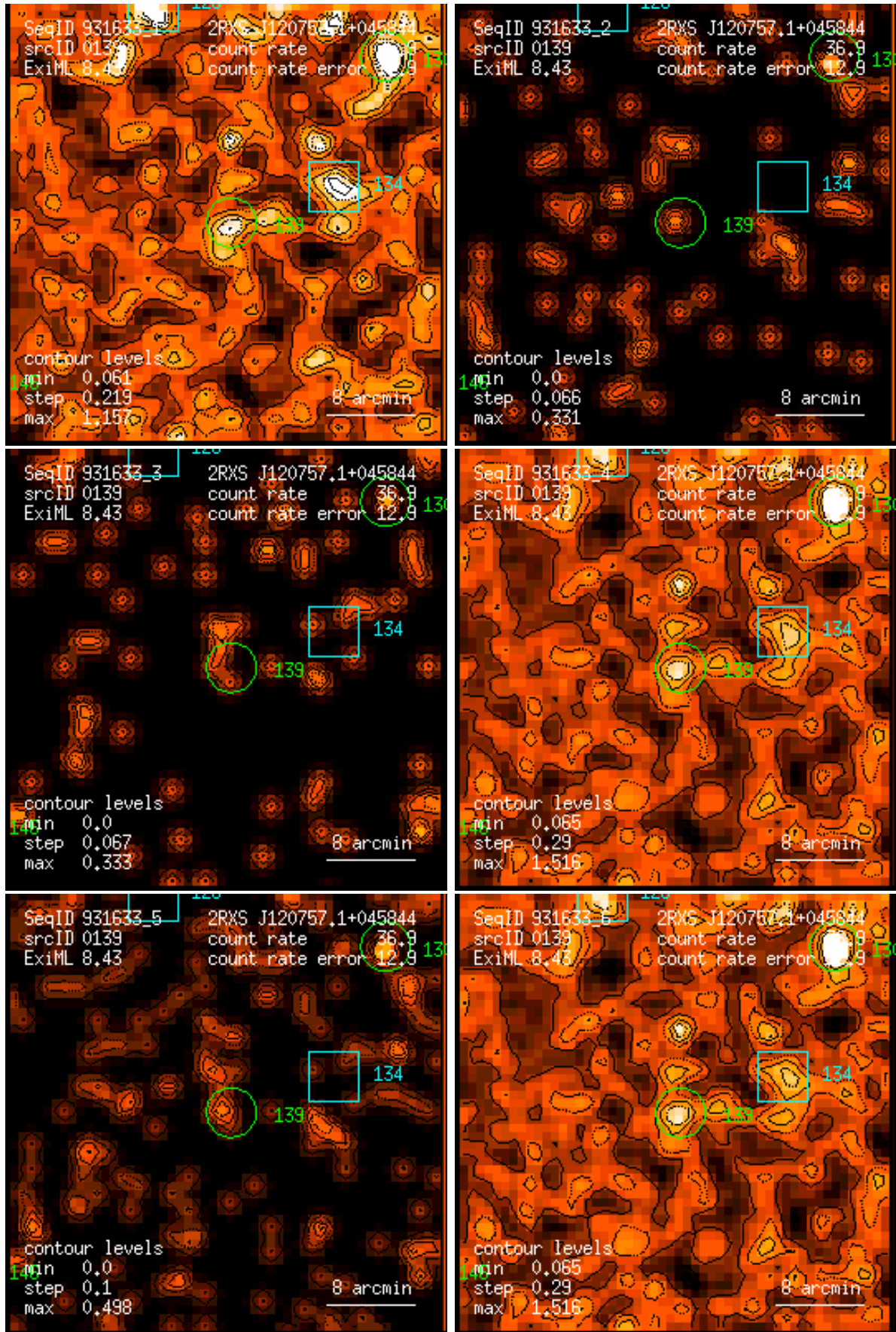
Figure 139: RASS 931633: detection 0139: band rate images, Gaussian filter: (1) PSPC channels 11 – 41, (2) 52 – 90, (3) 91 – 201, (4) 11 – 235, (5) 52 – 201, (6) 11 – 201. Broad band rates in counts/ks. Band rate contour levels in counts/ks/arcmin 2 .
