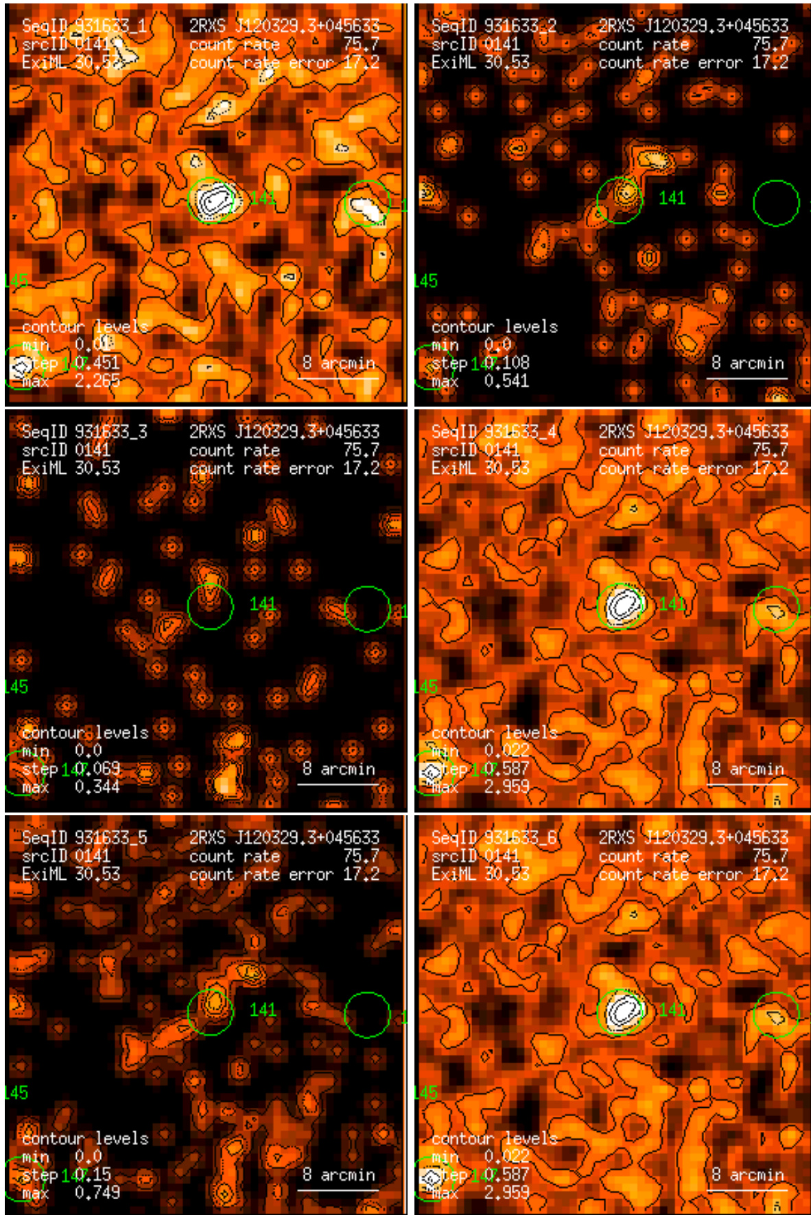
Figure 141: RASS 931633: detection 0141: band rate images, Gaussian filter: (1) PSPC channels 11 – 41, (2) 52 – 90, (3) 91 – 201, (4) 11 – 235, (5) 52 – 201, (6) 11 – 201. Broad band rates in counts/ks. Band rate contour levels in counts/ks/arcmin 2 .
