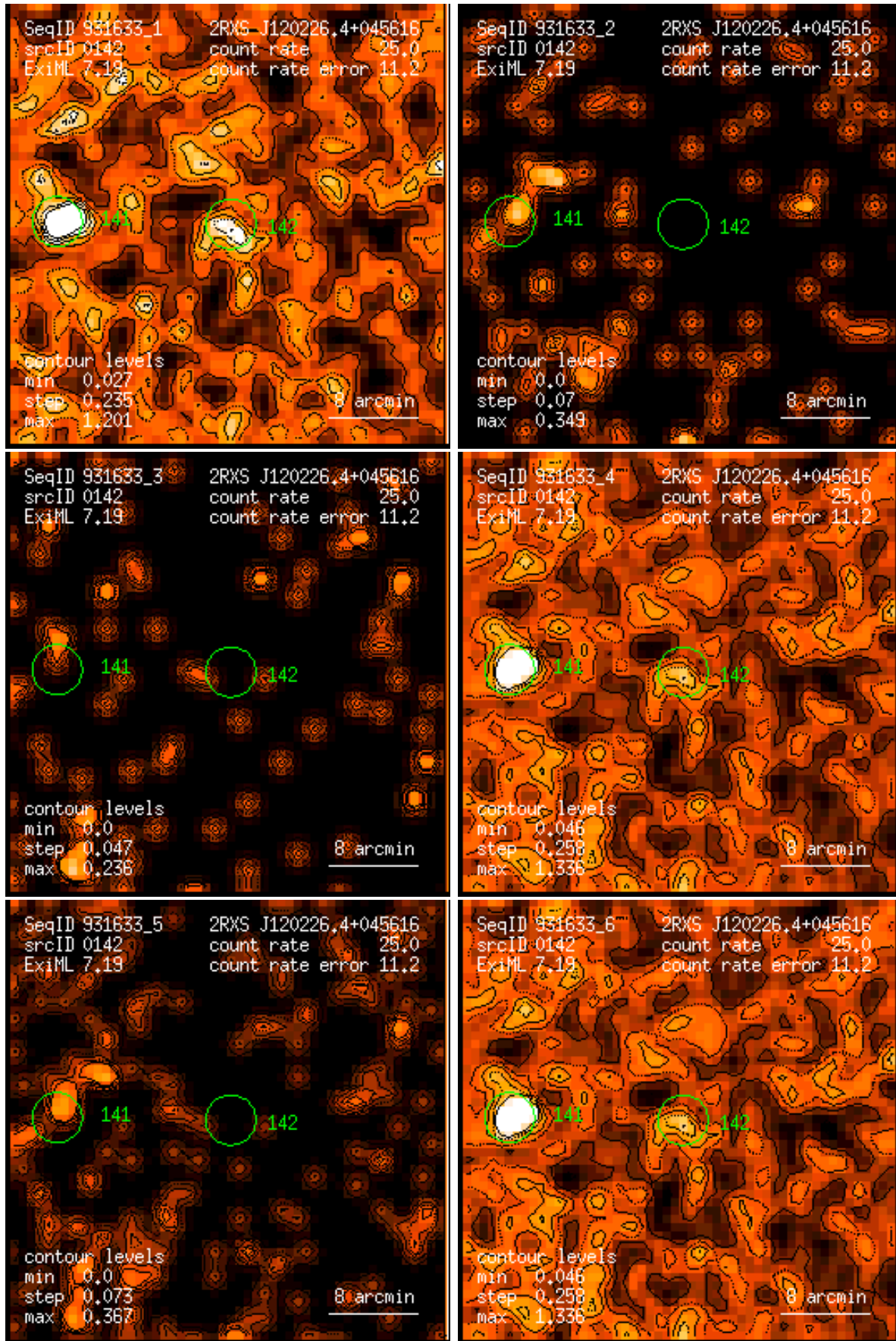
Figure 142: RASS 931633: detection 0142: band rate images, Gaussian filter: (1) PSPC channels 11 – 41, (2) 52 – 90, (3) 91 – 201, (4) 11 – 235, (5) 52 – 201, (6) 11 – 201. Broad band rates in counts/ks. Band rate contour levels in counts/ks/arcmin 2 .
