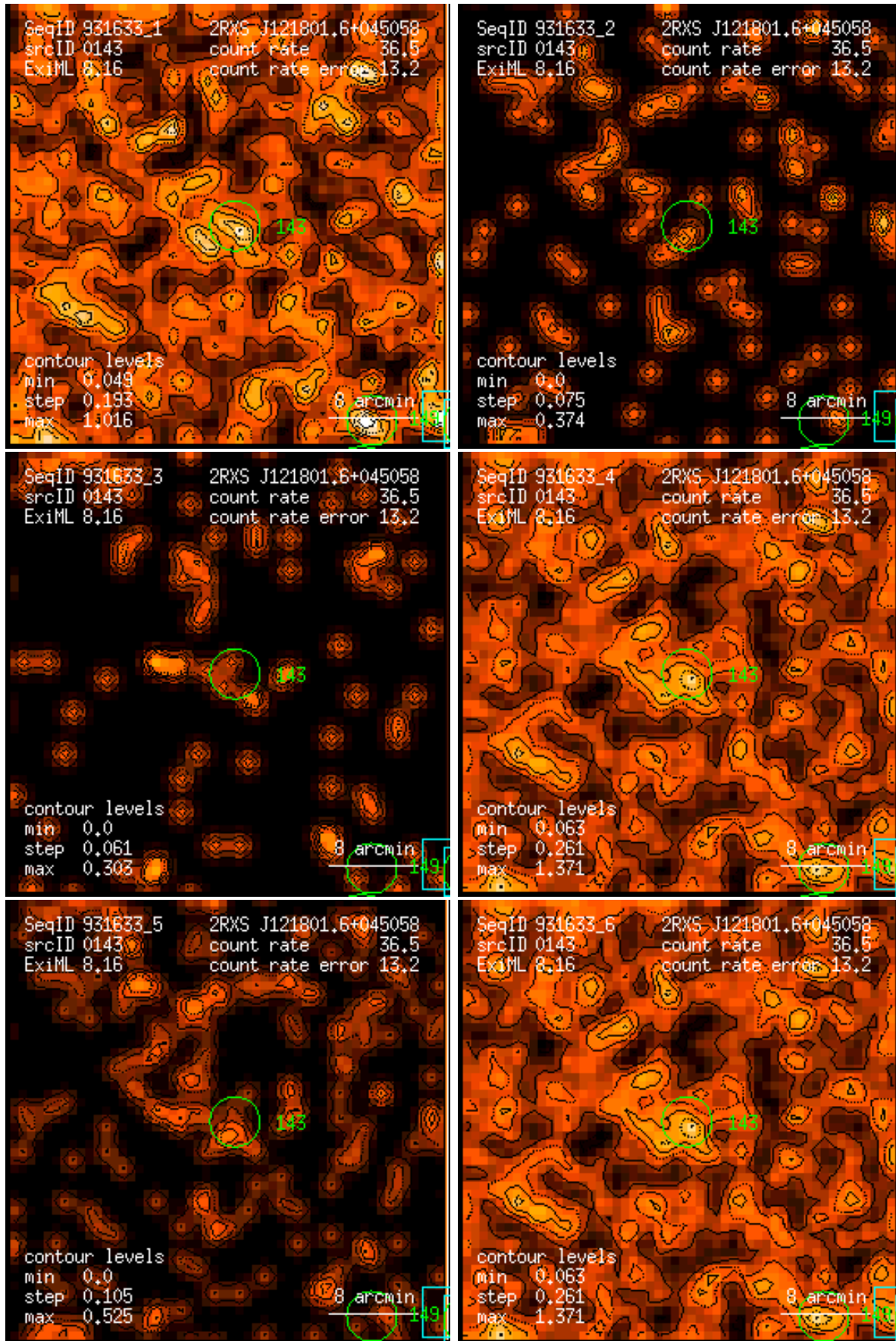
Figure 143: RASS 931633: detection 0143: band rate images, Gaussian filter: (1) PSPC channels 11 – 41, (2) 52 – 90, (3) 91 – 201, (4) 11 – 235, (5) 52 – 201, (6) 11 – 201. Broad band rates in counts/ks. Band rate contour levels in counts/ks/arcmin 2 .
