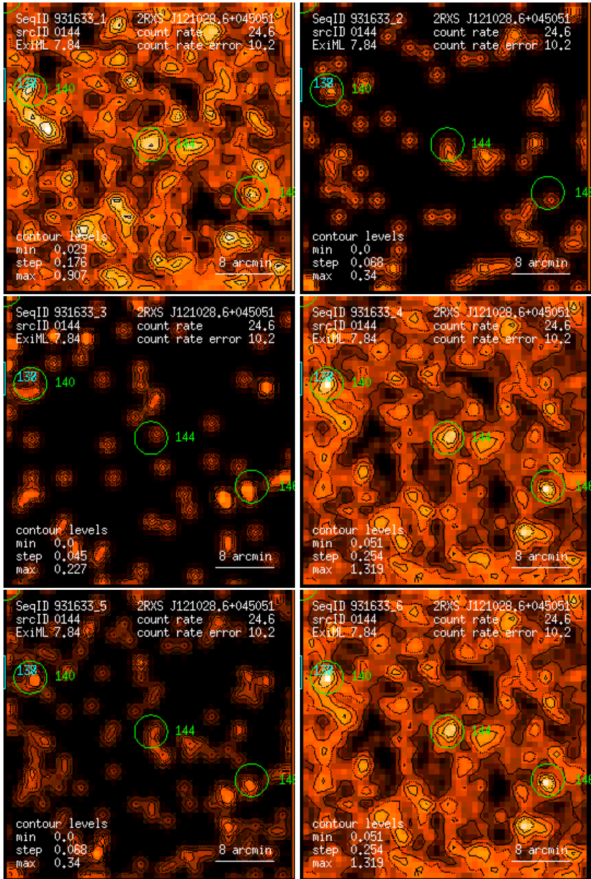
Figure 144: RASS 931633: detection 0144: band rate images, Gaussian filter: (1) PSPC channels 11 – 41, (2) 52 – 90, (3) 91 – 201, (4) 11 – 235, (5) 52 – 201, (6) 11 – 201. Broad band rates in counts/ks. Band rate contour levels in counts/ks/arcmin 2 .
