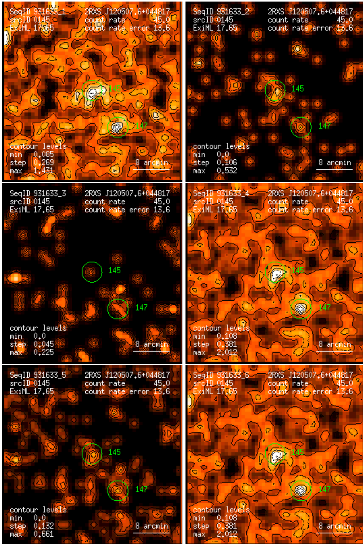
Figure 145: RASS 931633: detection 0145: band rate images, Gaussian filter: (1) PSPC channels 11 – 41, (2) 52 – 90, (3) 91 – 201, (4) 11 – 235, (5) 52 – 201, (6) 11 – 201. Broad band rates in counts/ks. Band rate contour levels in counts/ks/arcmin 2 .
