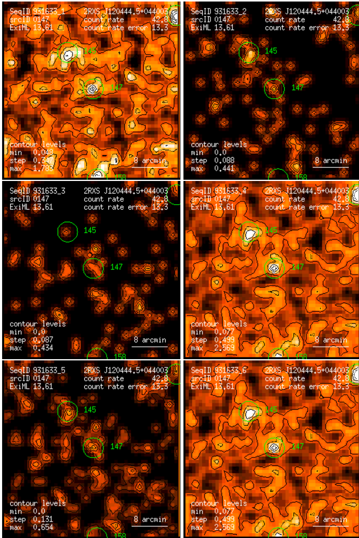
Figure 147: RASS 931633: detection 0147: band rate images, Gaussian filter: (1) PSPC channels 11 – 41, (2) 52 – 90, (3) 91 – 201, (4) 11 – 235, (5) 52 – 201, (6) 11 – 201. Broad band rates in counts/ks. Band rate contour levels in counts/ks/arcmin 2 .
