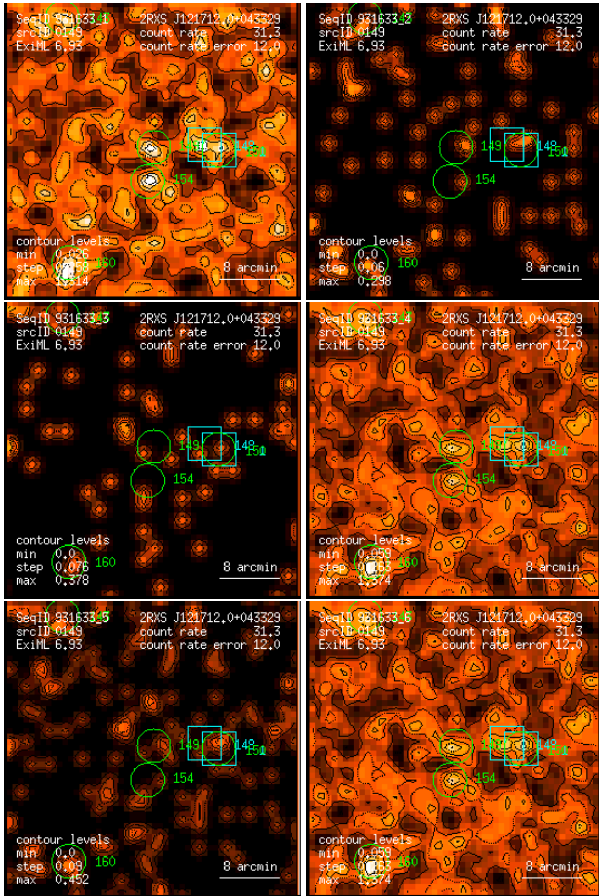
Figure 149: RASS 931633: detection 0149: band rate images, Gaussian filter: (1) PSPC channels 11 – 41, (2) 52 – 90, (3) 91 – 201, (4) 11 – 235, (5) 52 – 201, (6) 11 – 201. Broad band rates in counts/ks. Band rate contour levels in counts/ks/arcmin 2 .
