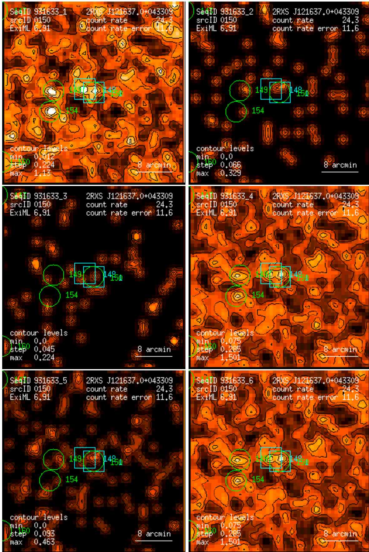
Figure 150: RASS 931633: detection 0150: band rate images, Gaussian filter: (1) PSPC channels 11 – 41, (2) 52 – 90, (3) 91 – 201, (4) 11 – 235, (5) 52 – 201, (6) 11 – 201. Broad band rates in counts/ks. Band rate contour levels in counts/ks/arcmin 2 .
