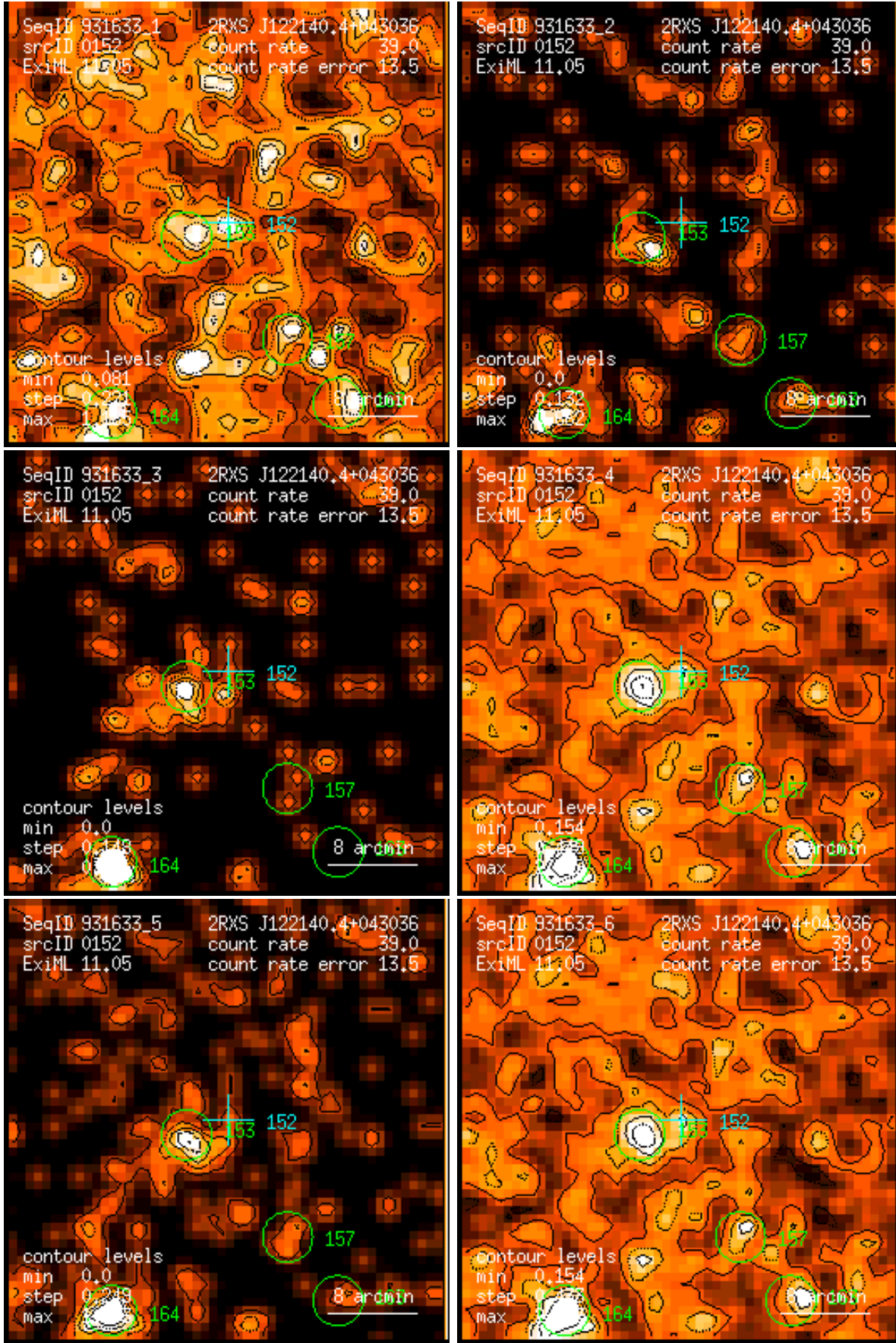
Figure 152: RASS 931633: detection 0152: band rate images, Gaussian filter: (1) PSPC channels 11 – 41, (2) 52 – 90, (3) 91 – 201, (4) 11 – 235, (5) 52 – 201, (6) 11 – 201. Broad band rates in counts/ks. Band rate contour levels in counts/ks/arcmin 2 .
