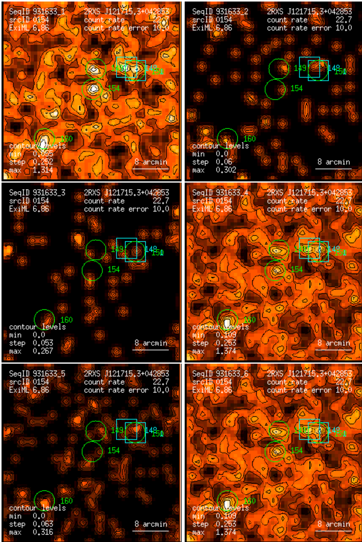
Figure 154: RASS 931633: detection 0154: band rate images, Gaussian filter: (1) PSPC channels 11 – 41, (2) 52 – 90, (3) 91 – 201, (4) 11 – 235, (5) 52 – 201, (6) 11 – 201. Broad band rates in counts/ks. Band rate contour levels in counts/ks/arcmin 2 .
