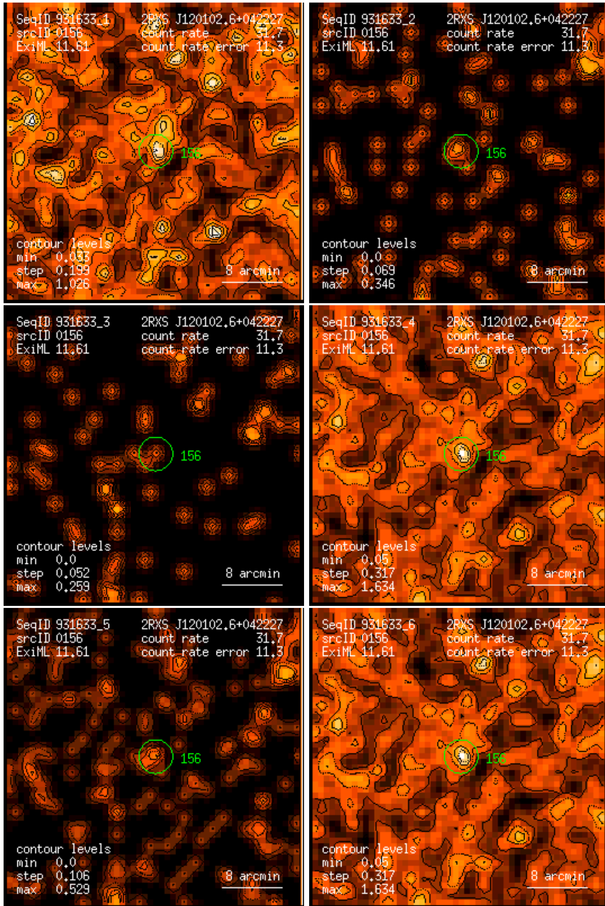
Figure 156: RASS 931633: detection 0156: band rate images, Gaussian filter: (1) PSPC channels 11 – 41, (2) 52 – 90, (3) 91 – 201, (4) 11 – 235, (5) 52 – 201, (6) 11 – 201. Broad band rates in counts/ks. Band rate contour levels in counts/ks/arcmin 2 .
