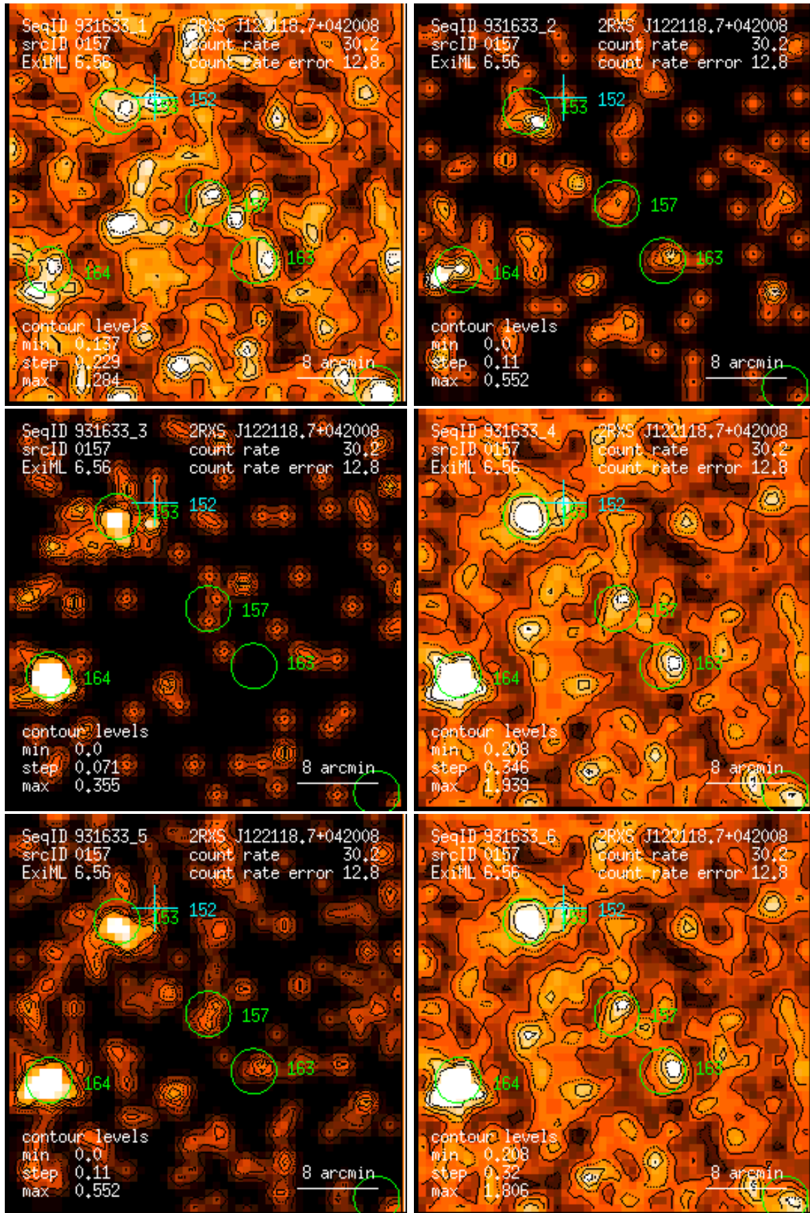
Figure 157: RASS 931633: detection 0157: band rate images, Gaussian filter: (1) PSPC channels 11 – 41, (2) 52 – 90, (3) 91 – 201, (4) 11 – 235, (5) 52 – 201, (6) 11 – 201. Broad band rates in counts/ks. Band rate contour levels in counts/ks/arcmin 2 .
