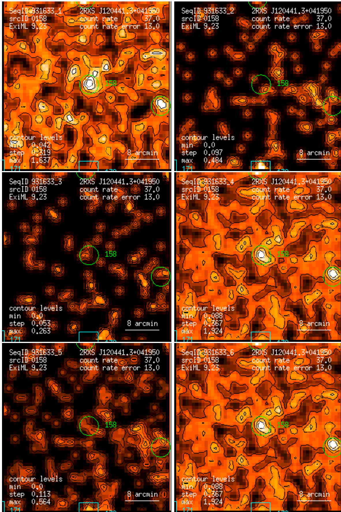
Figure 158: RASS 931633: detection 0158: band rate images, Gaussian filter: (1) PSPC channels 11 – 41, (2) 52 – 90, (3) 91 – 201, (4) 11 – 235, (5) 52 – 201, (6) 11 – 201. Broad band rates in counts/ks. Band rate contour levels in counts/ks/arcmin 2 .
