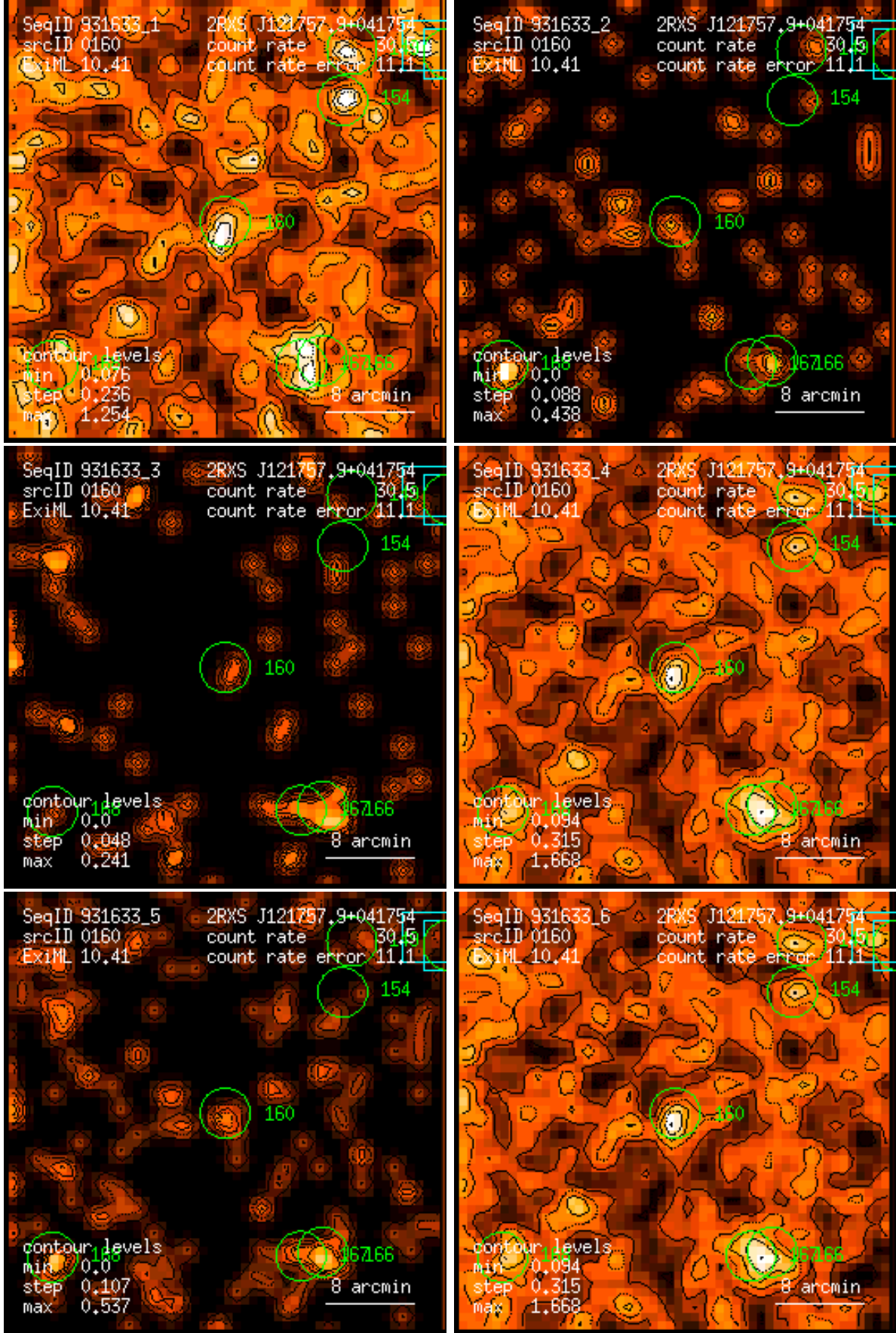
Figure 160: RASS 931633: detection 0160: band rate images, Gaussian filter: (1) PSPC channels 11 – 41, (2) 52 – 90, (3) 91 – 201, (4) 11 – 235, (5) 52 – 201, (6) 11 – 201. Broad band rates in counts/ks. Band rate contour levels in counts/ks/arcmin 2 .
