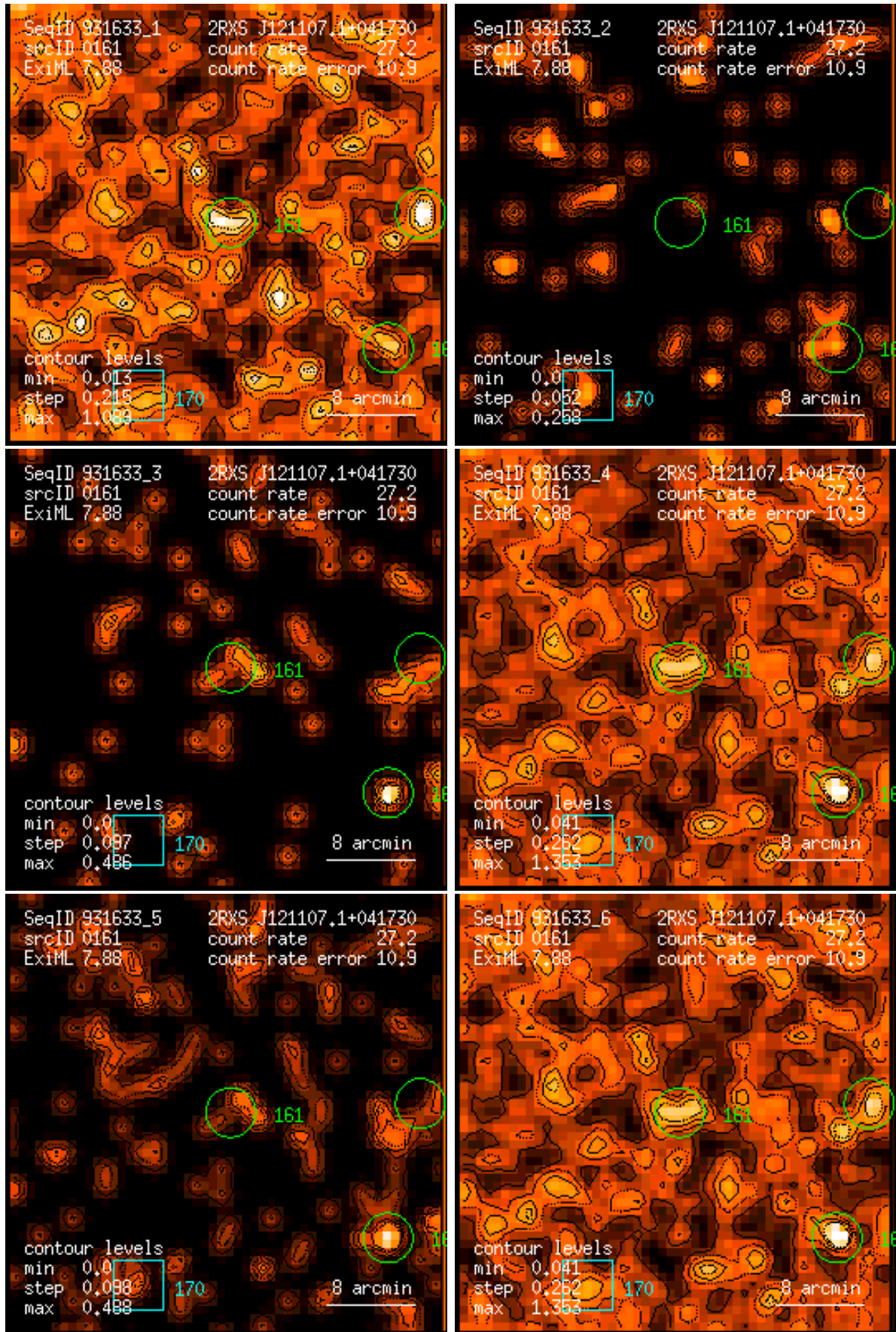
Figure 161: RASS 931633: detection 0161: band rate images, Gaussian filter: (1) PSPC channels 11 – 41, (2) 52 – 90, (3) 91 – 201, (4) 11 – 235, (5) 52 – 201, (6) 11 – 201. Broad band rates in counts/ks. Band rate contour levels in counts/ks/arcmin 2 .
