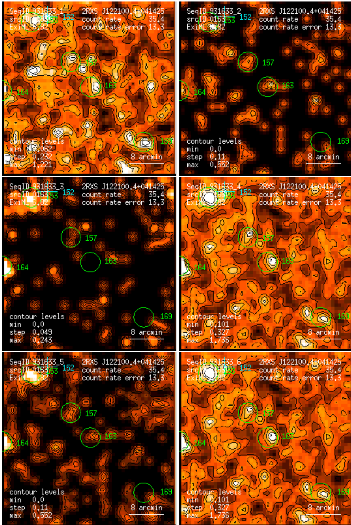
Figure 163: RASS 931633: detection 0163: band rate images, Gaussian filter: (1) PSPC channels 11 – 41, (2) 52 – 90, (3) 91 – 201, (4) 11 – 235, (5) 52 – 201, (6) 11 – 201. Broad band rates in counts/ks. Band rate contour levels in counts/ks/arcmin 2 .
