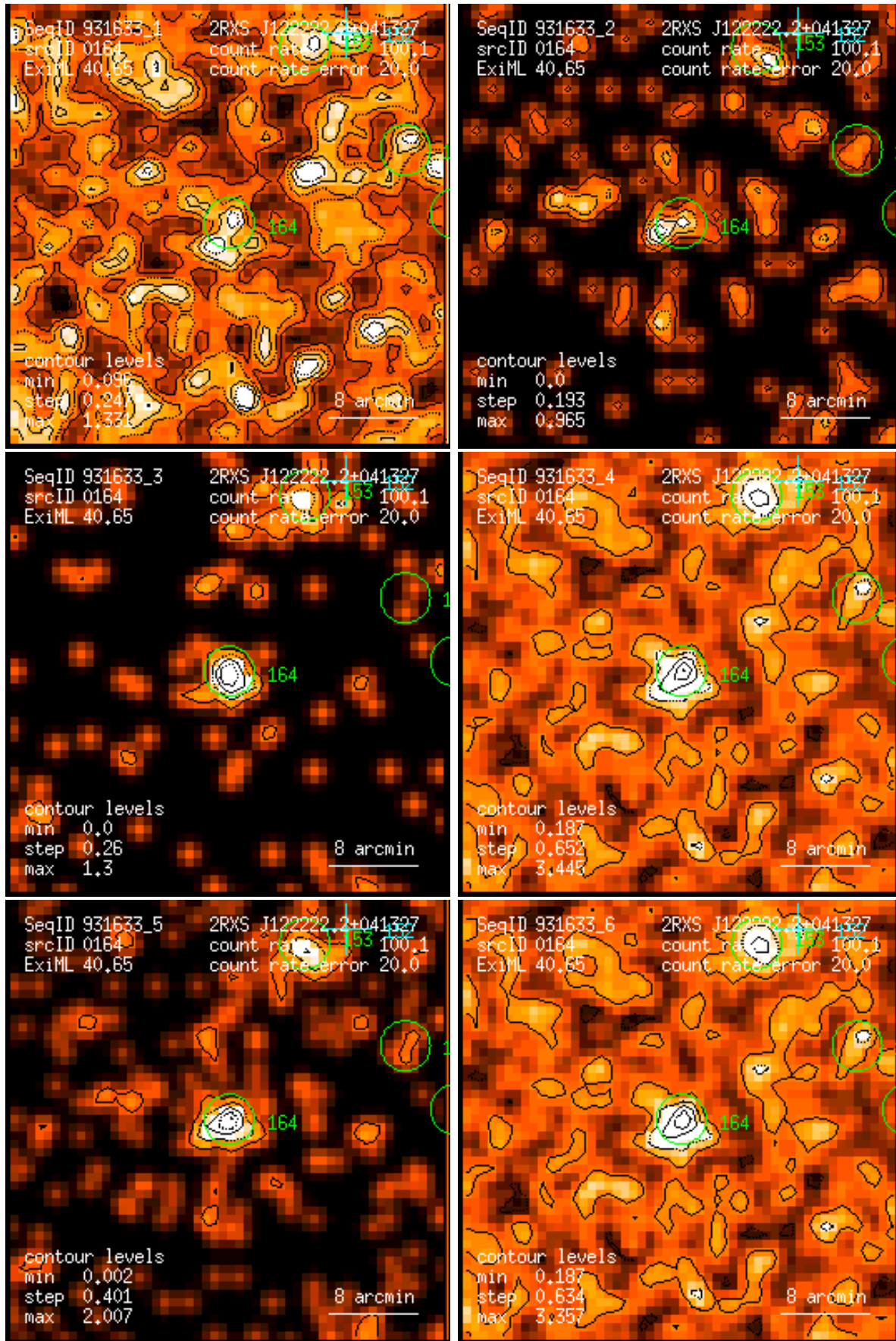
Figure 164: RASS 931633: detection 0164: band rate images, Gaussian filter: (1) PSPC channels 11 – 41, (2) 52 – 90, (3) 91 – 201, (4) 11 – 235, (5) 52 – 201, (6) 11 – 201. Broad band rates in counts/ks. Band rate contour levels in counts/ks/arcmin 2 .
