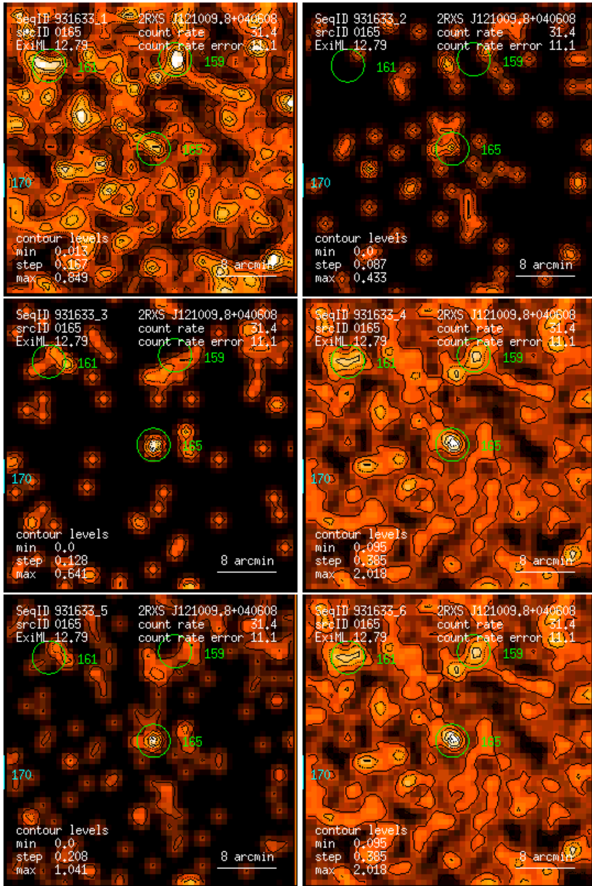
Figure 165: RASS 931633: detection 0165: band rate images, Gaussian filter: (1) PSPC channels 11 – 41, (2) 52 – 90, (3) 91 – 201, (4) 11 – 235, (5) 52 – 201, (6) 11 – 201. Broad band rates in counts/ks. Band rate contour levels in counts/ks/arcmin 2 .
