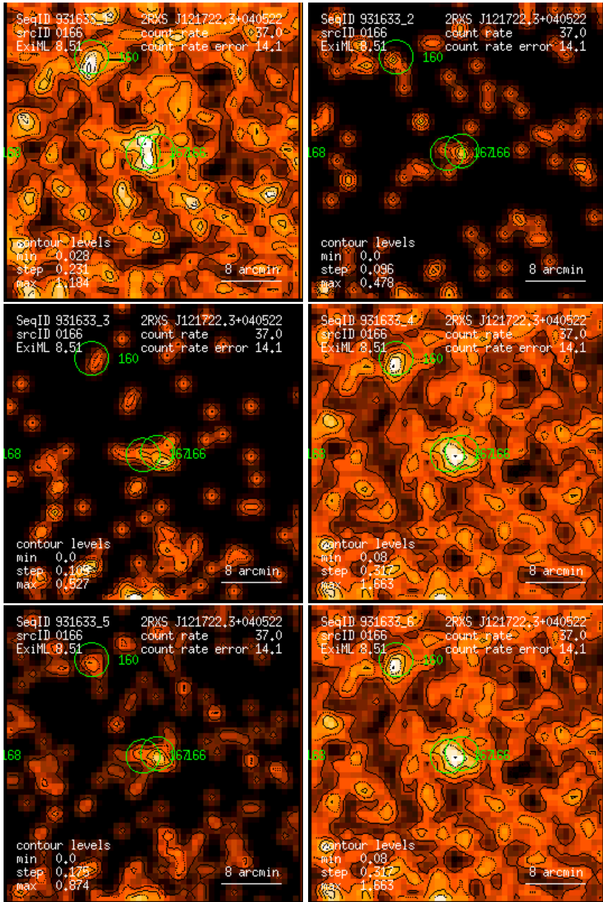
Figure 166: RASS 931633: detection 0166: band rate images, Gaussian filter: (1) PSPC channels 11 – 41, (2) 52 – 90, (3) 91 – 201, (4) 11 – 235, (5) 52 – 201, (6) 11 – 201. Broad band rates in counts/ks. Band rate contour levels in counts/ks/arcmin 2 .
