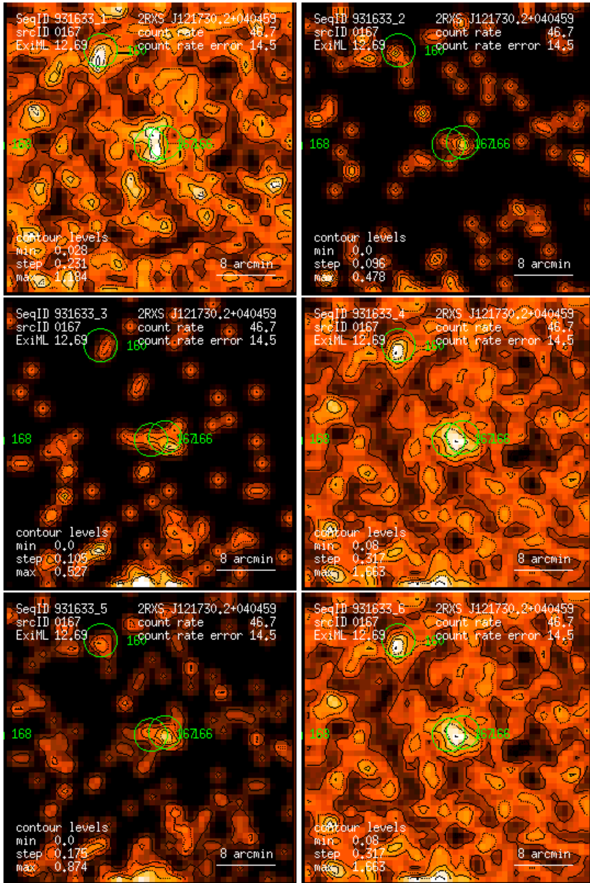
Figure 167: RASS 931633: detection 0167: band rate images, Gaussian filter: (1) PSPC channels 11 – 41, (2) 52 – 90, (3) 91 – 201, (4) 11 – 235, (5) 52 – 201, (6) 11 – 201. Broad band rates in counts/ks. Band rate contour levels in counts/ks/arcmin 2 .
