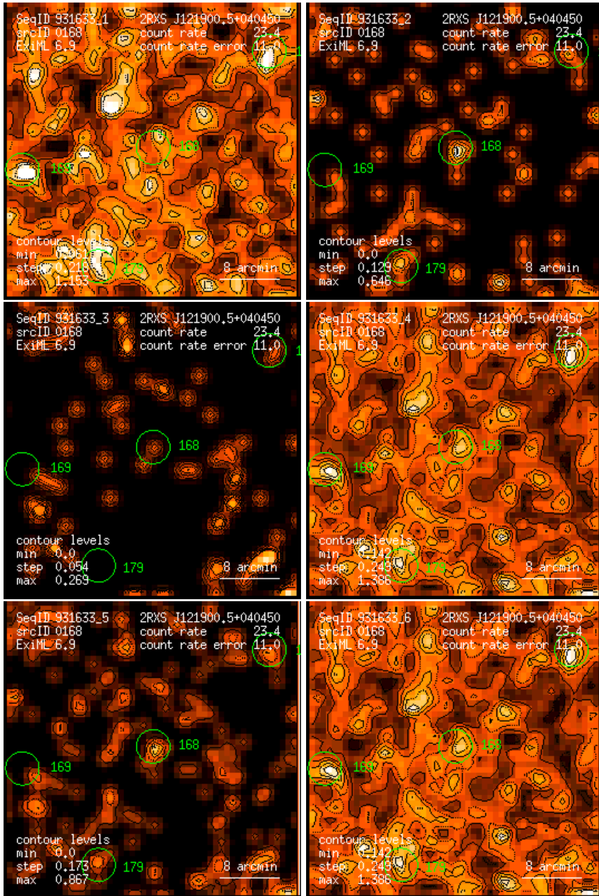
Figure 168: RASS 931633: detection 0168: band rate images, Gaussian filter: (1) PSPC channels 11 – 41, (2) 52 – 90, (3) 91 – 201, (4) 11 – 235, (5) 52 – 201, (6) 11 – 201. Broad band rates in counts/ks. Band rate contour levels in counts/ks/arcmin 2 .
