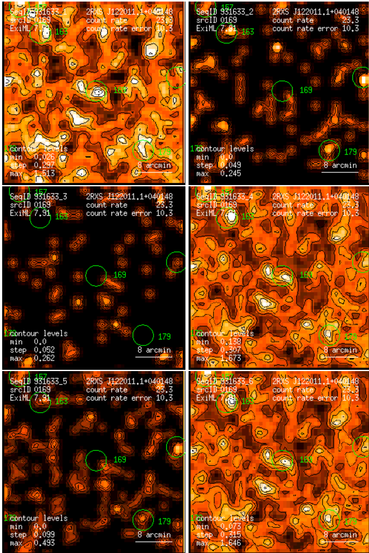
Figure 169: RASS 931633: detection 0169: band rate images, Gaussian filter: (1) PSPC channels 11 – 41, (2) 52 – 90, (3) 91 – 201, (4) 11 – 235, (5) 52 – 201, (6) 11 – 201. Broad band rates in counts/ks. Band rate contour levels in counts/ks/arcmin 2 .
