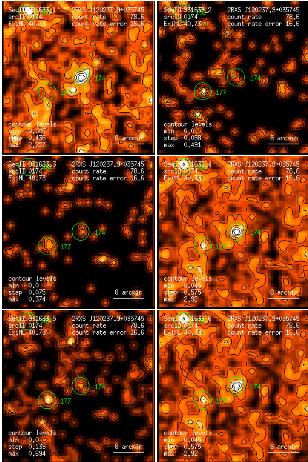
Figure 174: RASS 931633: detection 0174: band rate images, Gaussian filter: (1) PSPC channels 11 – 41, (2) 52 – 90, (3) 91 – 201, (4) 11 – 235, (5) 52 – 201, (6) 11 – 201. Broad band rates in counts/ks. Band rate contour levels in counts/ks/arcmin 2 .
