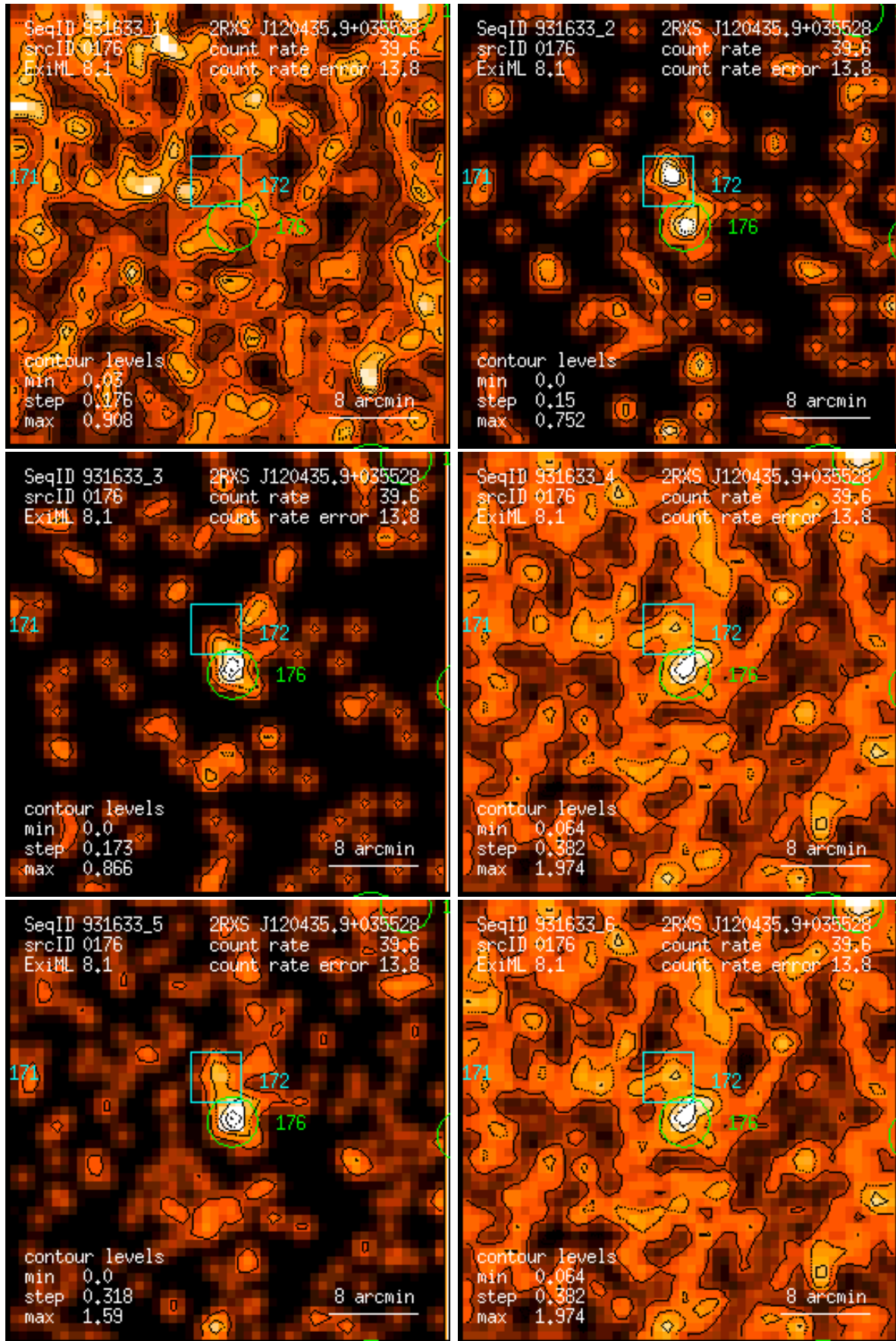
Figure 176: RASS 931633: detection 0176: band rate images, Gaussian filter: (1) PSPC channels 11 – 41, (2) 52 – 90, (3) 91 – 201, (4) 11 – 235, (5) 52 – 201, (6) 11 – 201. Broad band rates in counts/ks. Band rate contour levels in counts/ks/arcmin 2 .
