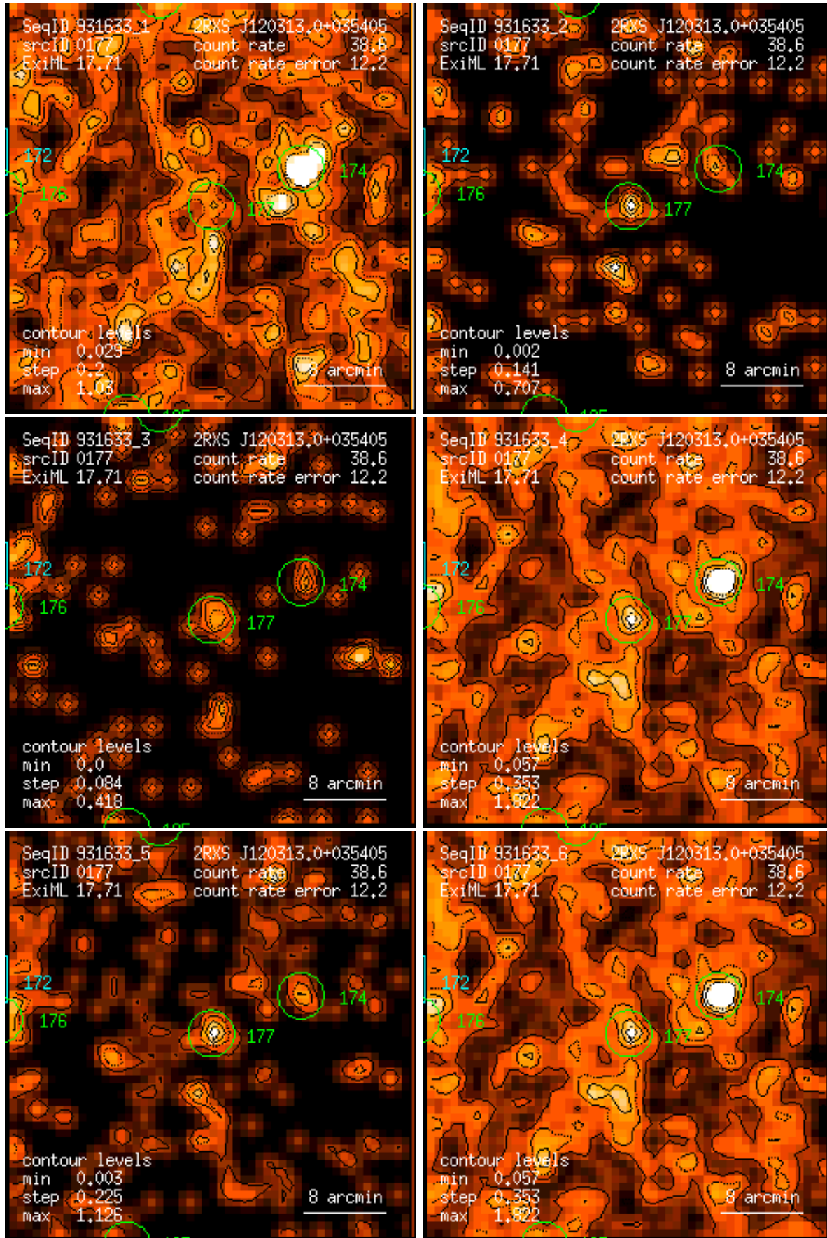
Figure 177: RASS 931633: detection 0177: band rate images, Gaussian filter: (1) PSPC channels 11 – 41, (2) 52 – 90, (3) 91 – 201, (4) 11 – 235, (5) 52 – 201, (6) 11 – 201. Broad band rates in counts/ks. Band rate contour levels in counts/ks/arcmin 2 .
