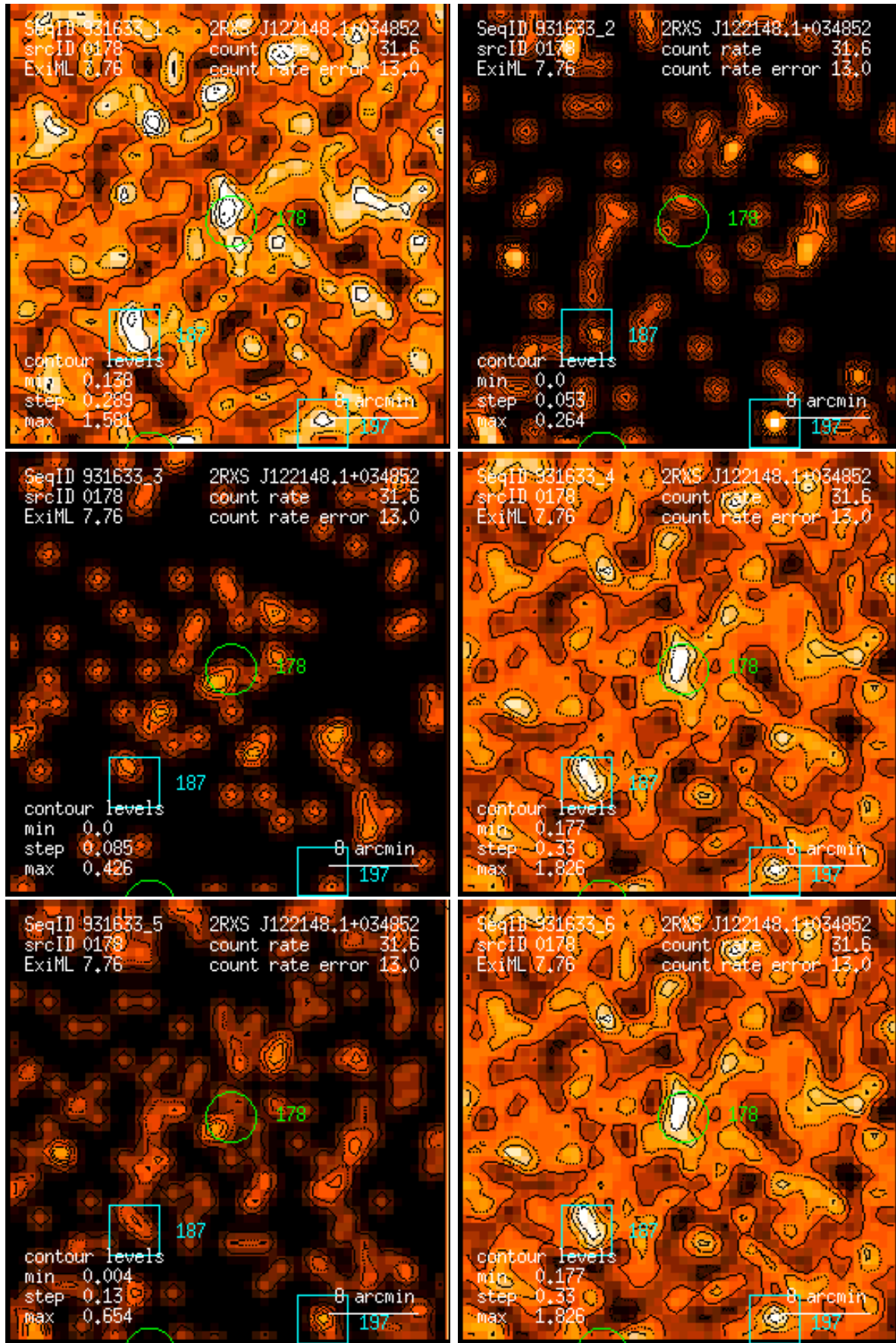
Figure 178: RASS 931633: detection 0178: band rate images, Gaussian filter: (1) PSPC channels 11 – 41, (2) 52 – 90, (3) 91 – 201, (4) 11 – 235, (5) 52 – 201, (6) 11 – 201. Broad band rates in counts/ks. Band rate contour levels in counts/ks/arcmin 2 .
