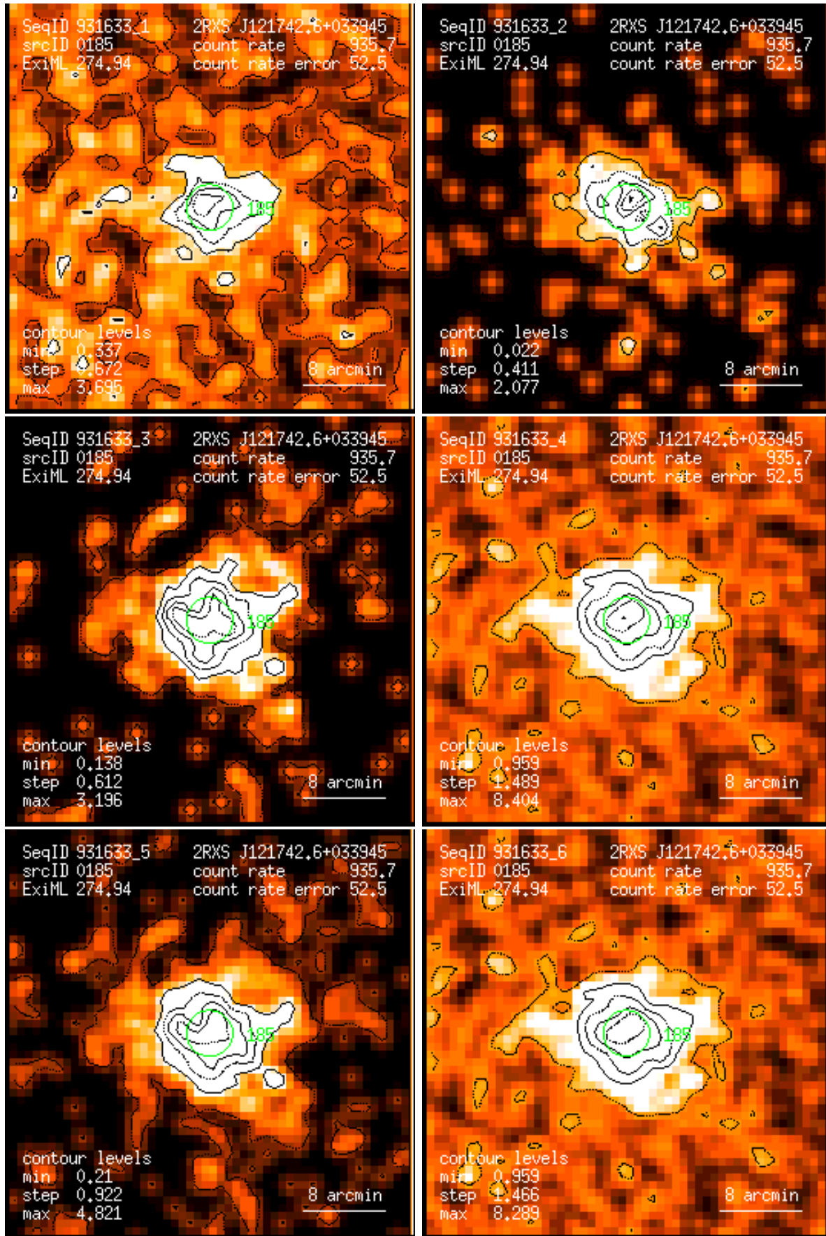
Figure 185: RASS 931633: detection 0185: band rate images, Gaussian filter: (1) PSPC channels 11 – 41, (2) 52 – 90, (3) 91 – 201, (4) 11 – 235, (5) 52 – 201, (6) 11 – 201. Broad band rates in counts/ks. Band rate contour levels in counts/ks/arcmin 2 .
