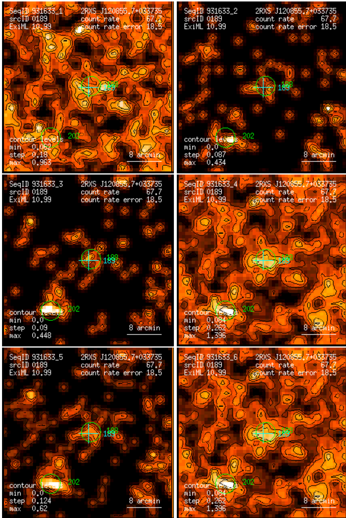
Figure 189: RASS 931633: detection 0189: band rate images, Gaussian filter: (1) PSPC channels 11 – 41, (2) 52 – 90, (3) 91 – 201, (4) 11 – 235, (5) 52 – 201, (6) 11 – 201. Broad band rates in counts/ks. Band rate contour levels in counts/ks/arcmin 2 .
