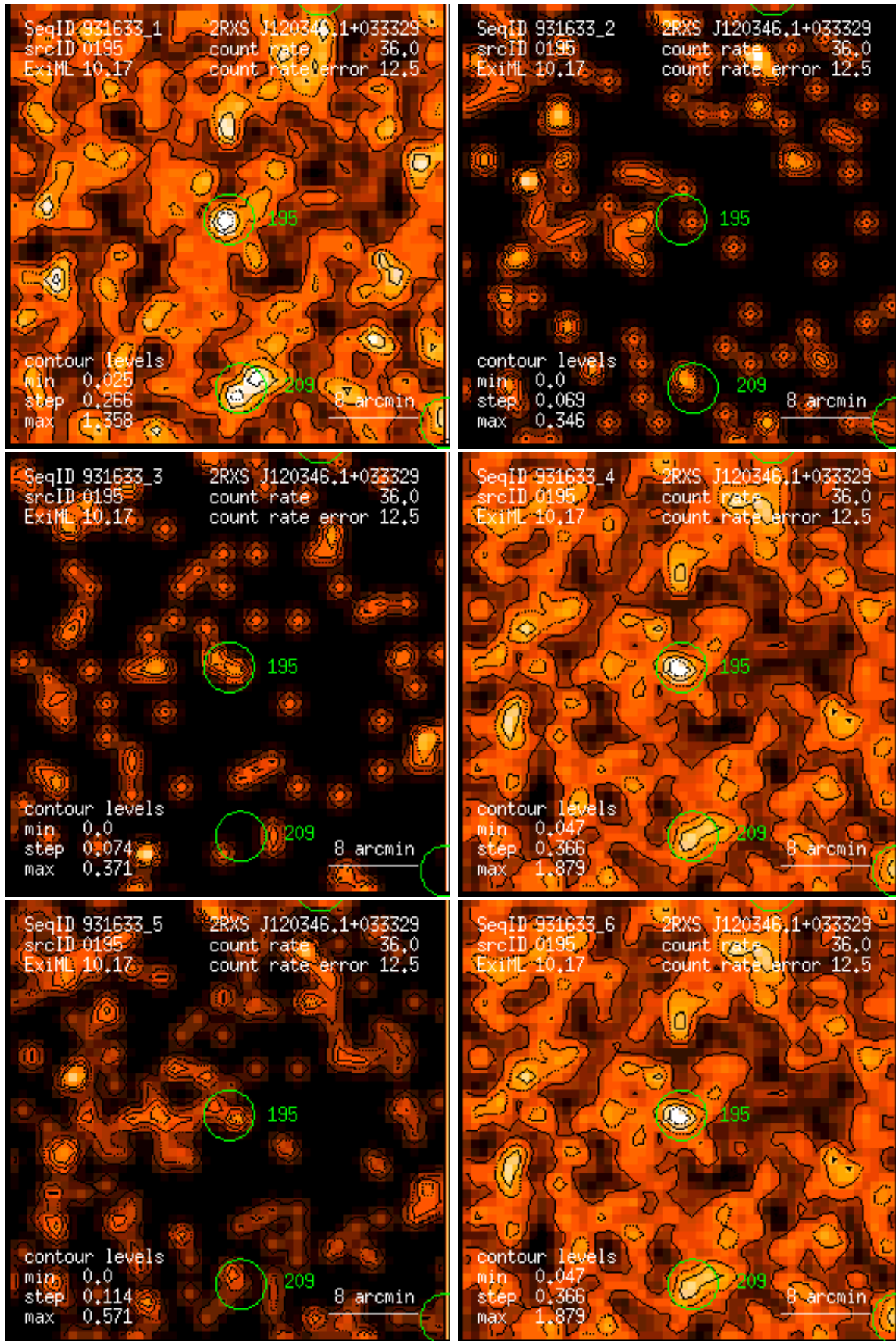
Figure 195: RASS 931633: detection 0195: band rate images, Gaussian filter: (1) PSPC channels 11 – 41, (2) 52 – 90, (3) 91 – 201, (4) 11 – 235, (5) 52 – 201, (6) 11 – 201. Broad band rates in counts/ks. Band rate contour levels in counts/ks/arcmin 2 .
