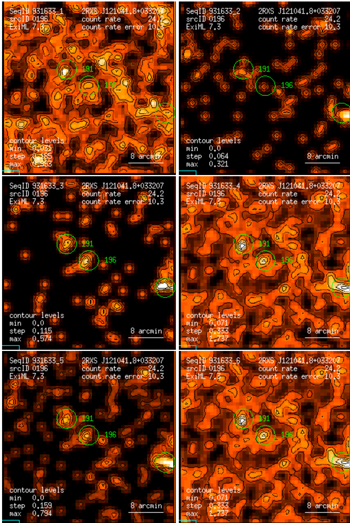
Figure 196: RASS 931633: detection 0196: band rate images, Gaussian filter: (1) PSPC channels 11 – 41, (2) 52 – 90, (3) 91 – 201, (4) 11 – 235, (5) 52 – 201, (6) 11 – 201. Broad band rates in counts/ks. Band rate contour levels in counts/ks/arcmin 2 .
