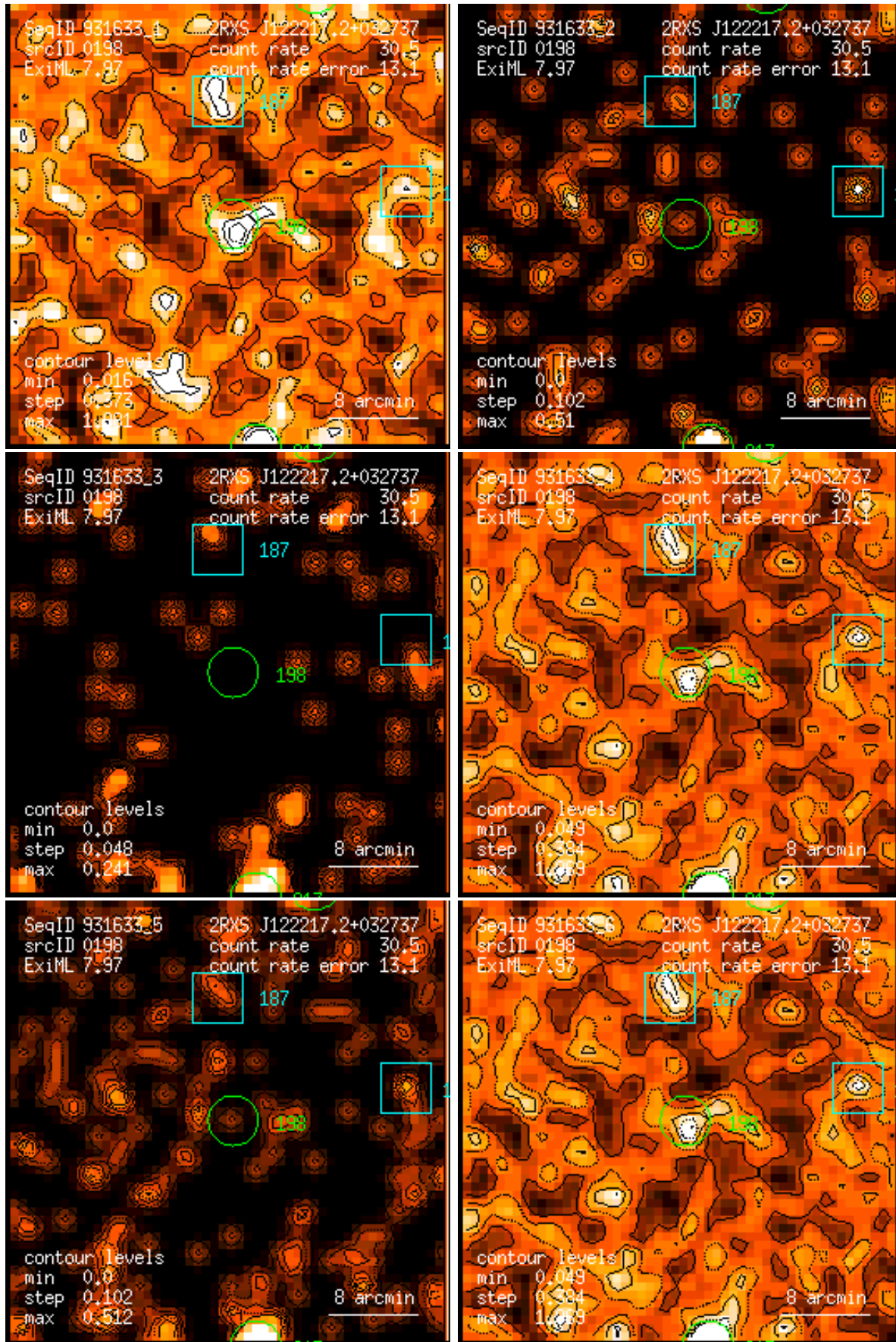
Figure 198: RASS 931633: detection 0198: band rate images, Gaussian filter: (1) PSPC channels 11 – 41, (2) 52 – 90, (3) 91 – 201, (4) 11 – 235, (5) 52 – 201, (6) 11 – 201. Broad band rates in counts/ks. Band rate contour levels in counts/ks/arcmin 2 .
