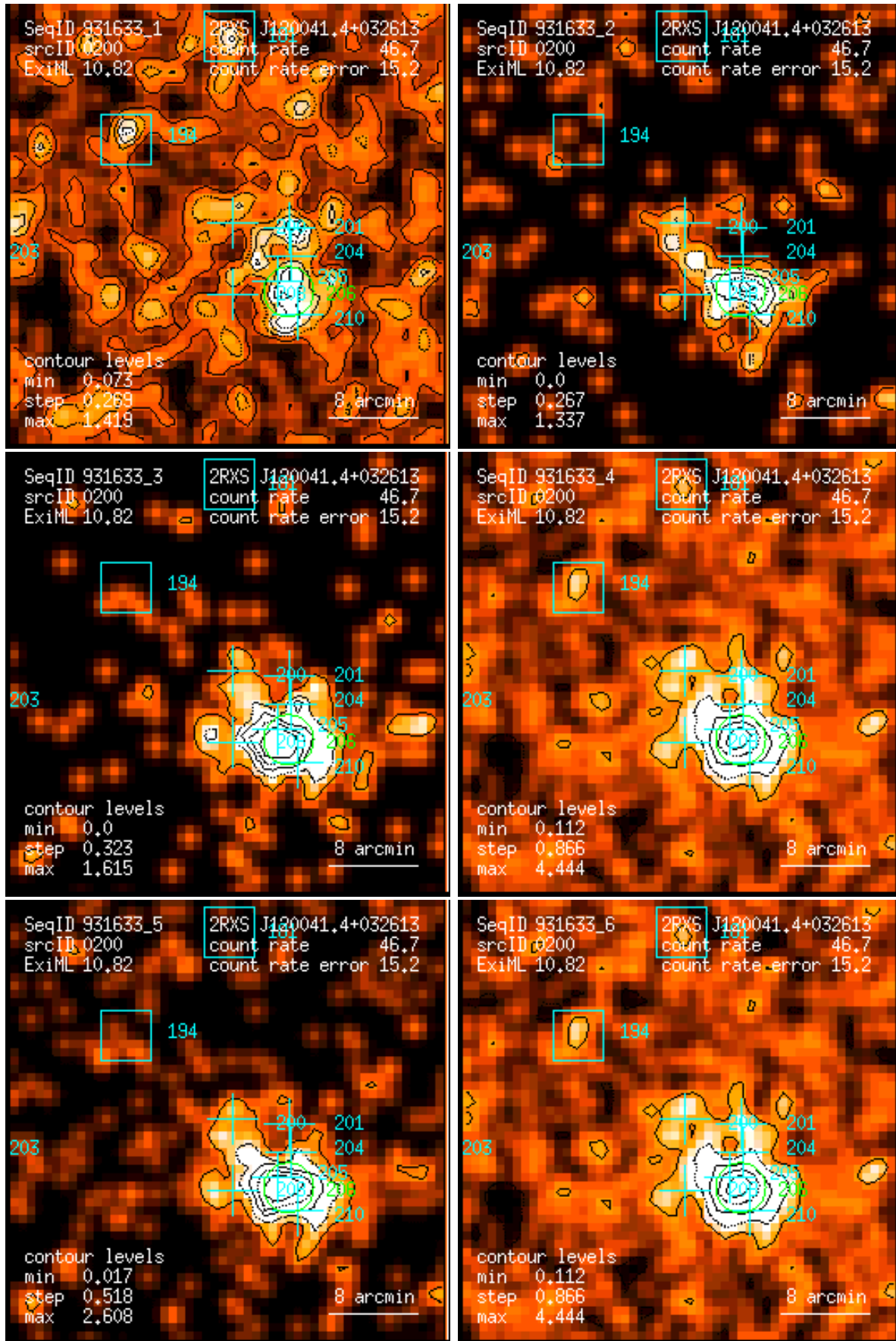
Figure 200: RASS 931633: detection 0200: band rate images, Gaussian filter: (1) PSPC channels 11 – 41, (2) 52 – 90, (3) 91 – 201, (4) 11 – 235, (5) 52 – 201, (6) 11 – 201. Broad band rates in counts/ks. Band rate contour levels in counts/ks/arcmin 2 .
