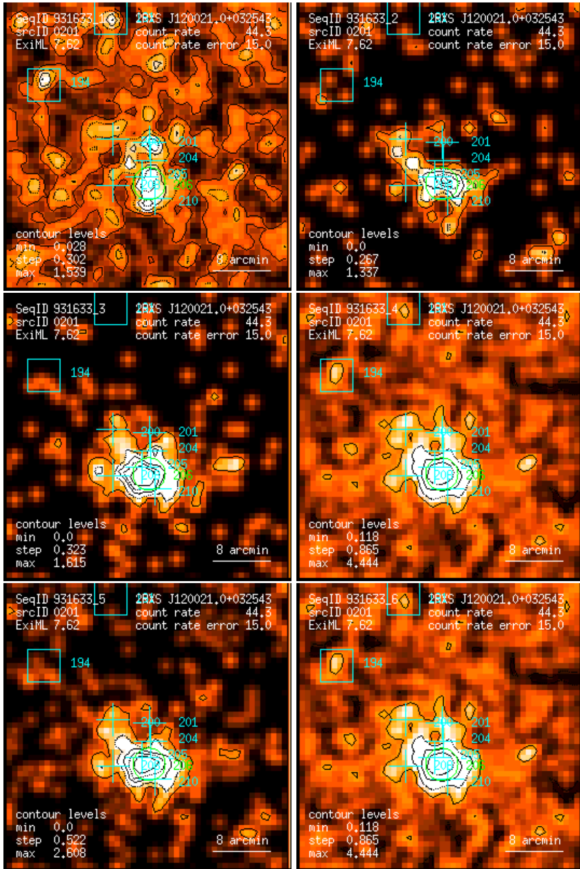
Figure 201: RASS 931633: detection 0201: band rate images, Gaussian filter: (1) PSPC channels 11 – 41, (2) 52 – 90, (3) 91 – 201, (4) 11 – 235, (5) 52 – 201, (6) 11 – 201. Broad band rates in counts/ks. Band rate contour levels in counts/ks/arcmin 2 .
