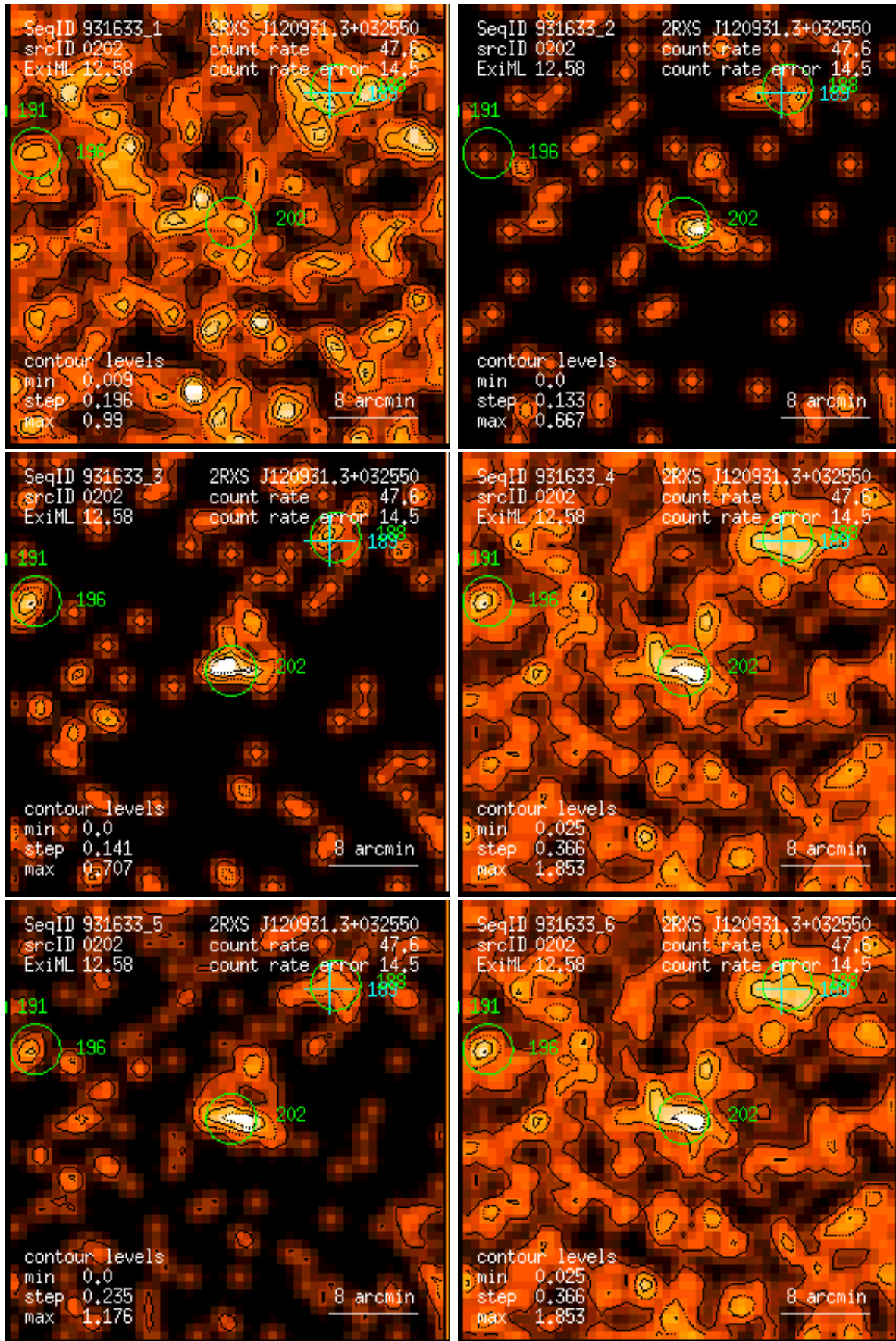
Figure 202: RASS 931633: detection 0202: band rate images, Gaussian filter: (1) PSPC channels 11 – 41, (2) 52 – 90, (3) 91 – 201, (4) 11 – 235, (5) 52 – 201, (6) 11 – 201. Broad band rates in counts/ks. Band rate contour levels in counts/ks/arcmin 2 .
