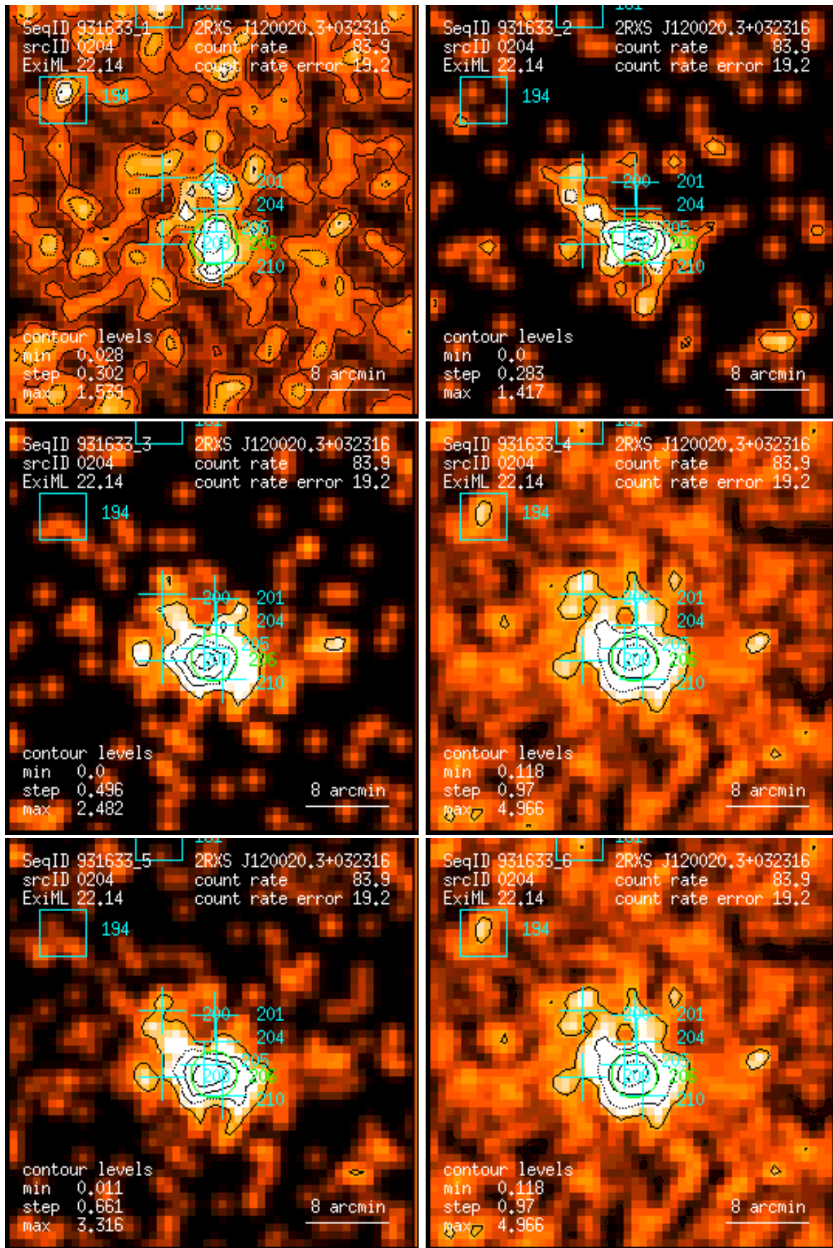
Figure 204: RASS 931633: detection 0204: band rate images, Gaussian filter: (1) PSPC channels 11 – 41, (2) 52 – 90, (3) 91 – 201, (4) 11 – 235, (5) 52 – 201, (6) 11 – 201. Broad band rates in counts/ks. Band rate contour levels in counts/ks/arcmin 2 .
