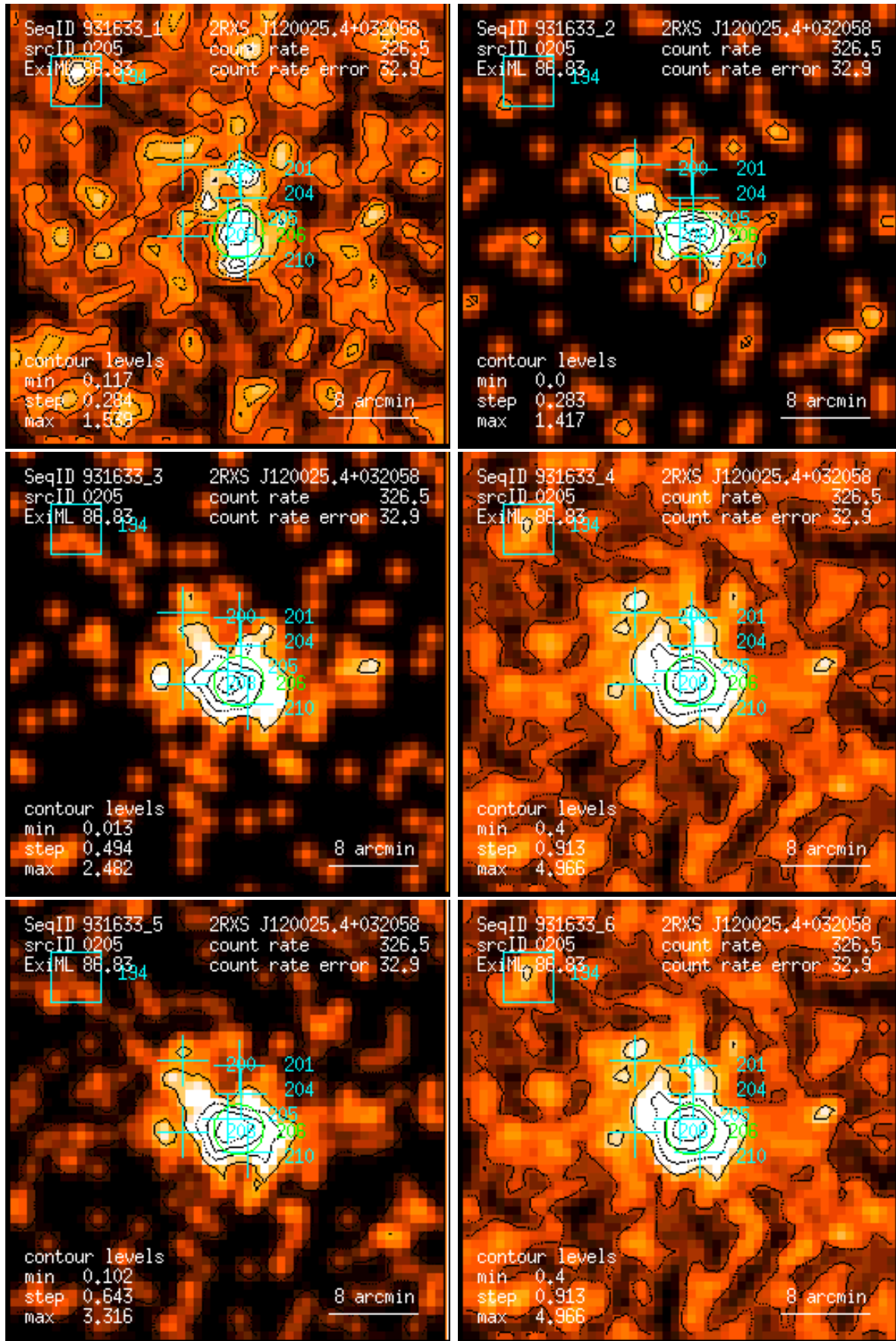
Figure 205: RASS 931633: detection 0205: band rate images, Gaussian filter: (1) PSPC channels 11 – 41, (2) 52 – 90, (3) 91 – 201, (4) 11 – 235, (5) 52 – 201, (6) 11 – 201. Broad band rates in counts/ks. Band rate contour levels in counts/ks/arcmin 2 .
