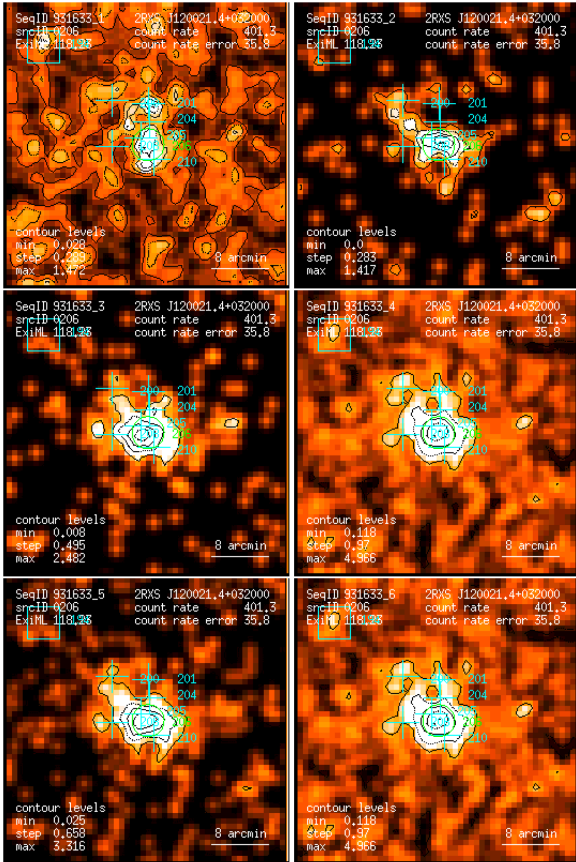
Figure 206: RASS 931633: detection 0206: band rate images, Gaussian filter: (1) PSPC channels 11 – 41, (2) 52 – 90, (3) 91 – 201, (4) 11 – 235, (5) 52 – 201, (6) 11 – 201. Broad band rates in counts/ks. Band rate contour levels in counts/ks/arcmin 2 .
