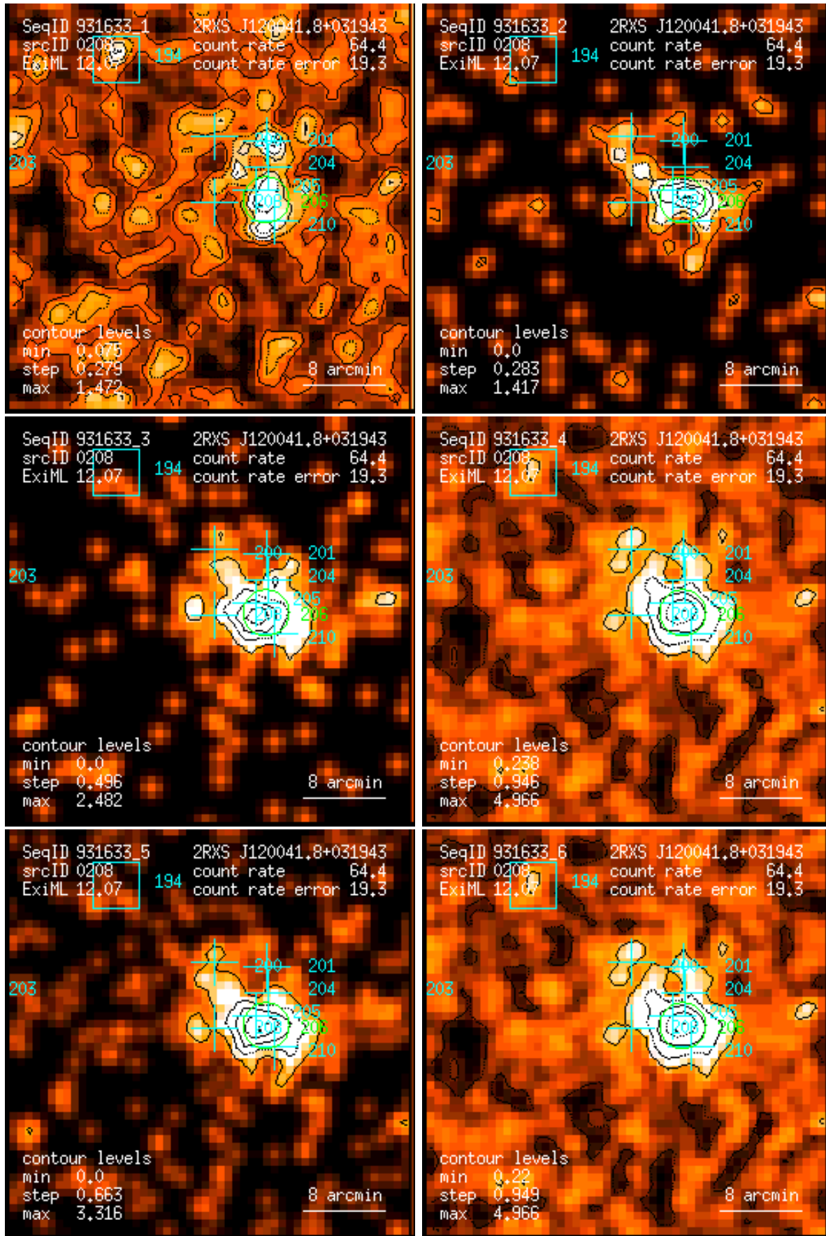
Figure 208: RASS 931633: detection 0208: band rate images, Gaussian filter: (1) PSPC channels 11 – 41, (2) 52 – 90, (3) 91 – 201, (4) 11 – 235, (5) 52 – 201, (6) 11 – 201. Broad band rates in counts/ks. Band rate contour levels in counts/ks/arcmin 2 .
